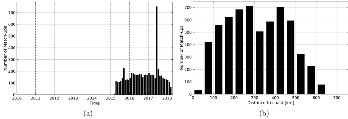
Figure 1: Number of match-ups between Argo and SMAP-L3-RSS-V2-8DAY-RUNNING-70KM SSS as a function of time (a) and as function of the distance to coast (b) over the Bay of Bengal Pi-MEP region and for the full satellite product period.
