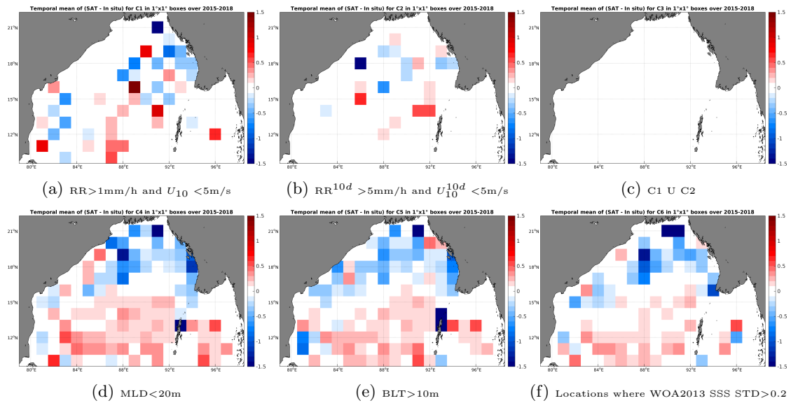
Figure 12: Temporal mean gridded over spatial boxes of size 1^\circ \times 1^\circ of \Delta SSS (SMAP-L3-RSS-V2-8DAY-RUNNING-70KM - Argo) for 6 different subdatasets corresponding to: RR > 1\text{mm/h} and U_{10} < 5\text{m/s} (a), RR^{10d} > 5\text{mm/h} and U_{10}^{10d} < 5\text{m/s} (b), C1 U C2 (c), MLD < 20\text{m} (d), BLT > 10\text{m} (e), Locations where WOA2013 SSS STD > 0.2 (f).
