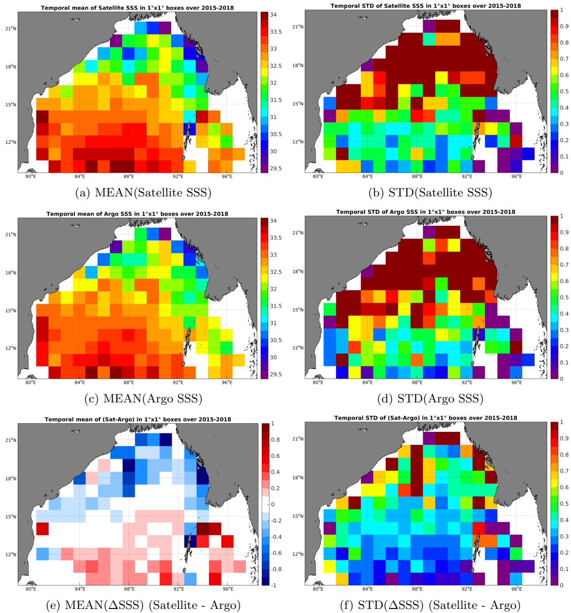
Figure 6: Temporal mean (left) and STD (right) of SSS from SMAP-L3-RSS-V2-8DAY-RUNNING-70KM (top), Argo (middle), and of \Delta SSS (Satellite - Argo). Only match-up pairs are used to generate these maps.
