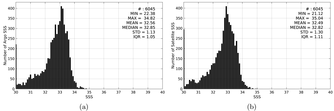
Figure 2: Histograms of SSS from Argo (a) and SMAP-L3-RSS-V2-8DAY-RUNNING-70KM (b) considering all match-up pairs per bins of 0.1 over the Bay of Bengal Pi-MEP region and for the full satellite product period.
