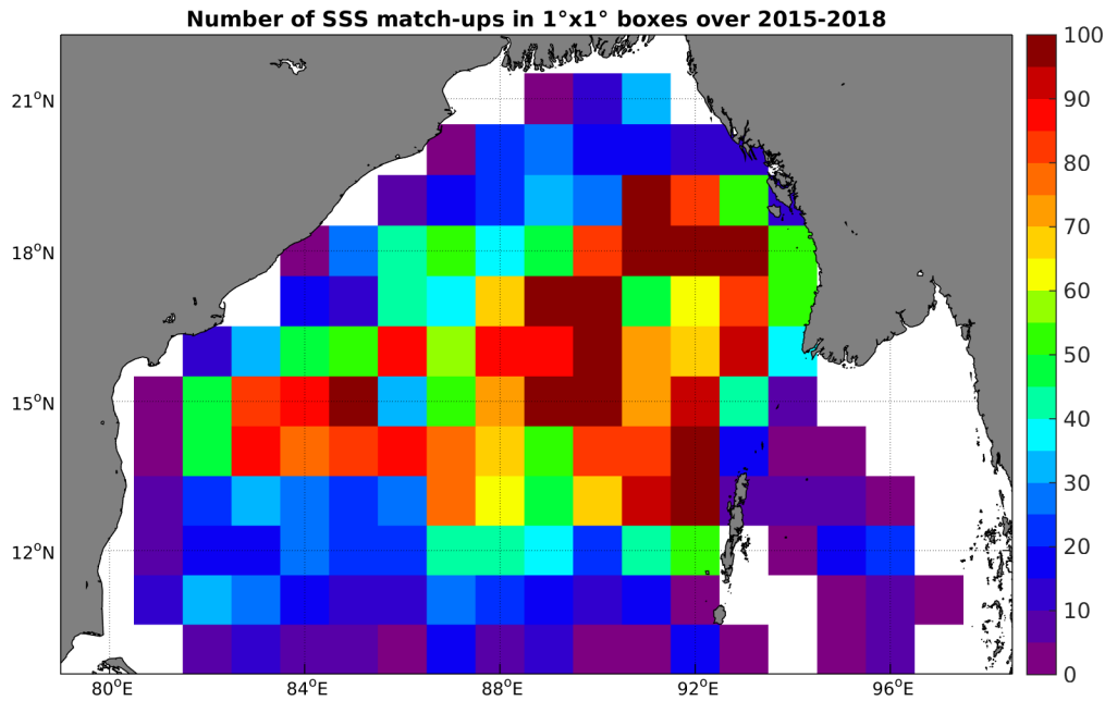
Figure 4: Number of SSS match-ups between Argo SSS and the SMAP-L3-RSS-V2-8DAY-RUNNING-70KM SSS product for the Bay of Bengal Pi-MEP region over 1^{\circ} \times 1^{\circ} boxes and for the full satellite product period.
