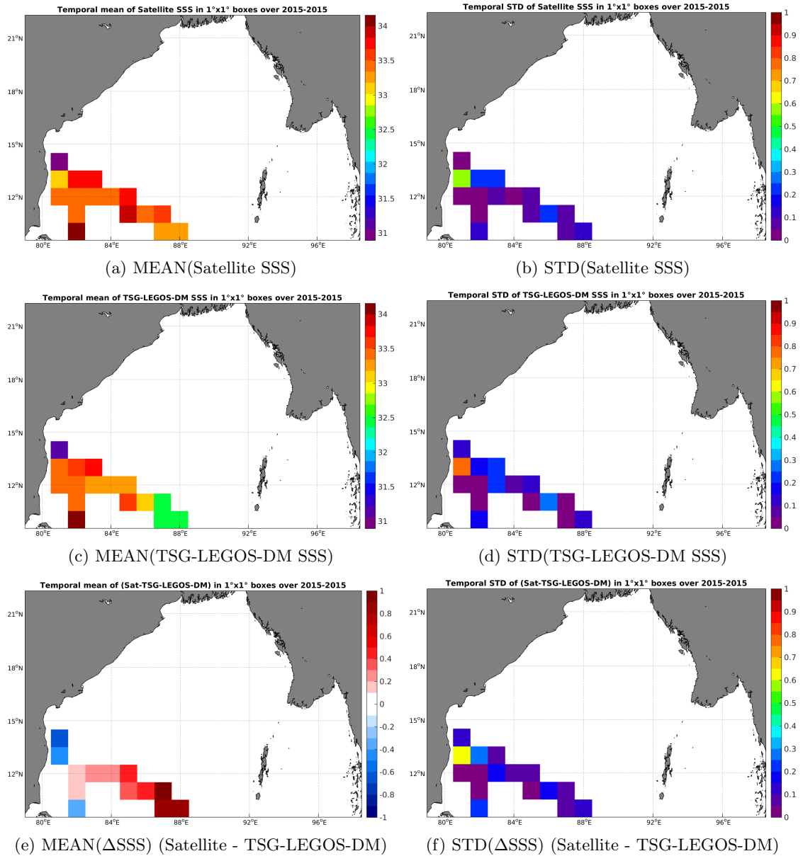
Figure 6: Temporal mean (left) and STD (right) of SSS from SMAP-L3-RSS-V2-MONTHLY-0.25DEG-40KM (top), TSG-LEGOS-DM (middle), and of \Delta SSS (Satellite - TSG-LEGOS-DM). Only match-up pairs are used to generate these maps.
