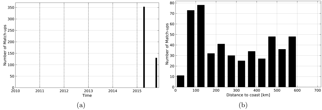
Figure 1: Number of match-ups between TSG-LEGOS-DM and SMAP-L3-RSS-V2-MONTHLY-0.25DEG-40KM SSS as a function of time (a) and as function of the distance to coast (b) over the Bay of Bengal Pi-MEP region and for the full satellite product period.
