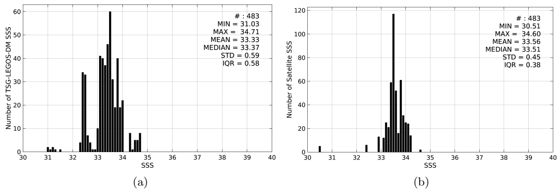
Figure 2: Histograms of SSS from TSG-LEGOS-DM (a) and SMAP-L3-RSS-V2-MONTHLY-0.25DEG-40KM (b) considering all match-up pairs per bins of 0.1 over the Bay of Bengal Pi-MEP region and for the full satellite product period.
