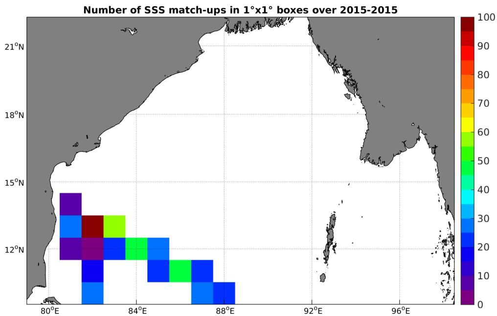
Figure 4: Number of SSS match-ups between TSG-LEGOS-DM SSS and the SMAP-L3-RSS-V2-MONTHLY-0.25DEG-40KM SSS product for the Bay of Bengal Pi-MEP region over 1^\circ \times 1^\circ boxes and for the full satellite product period.
