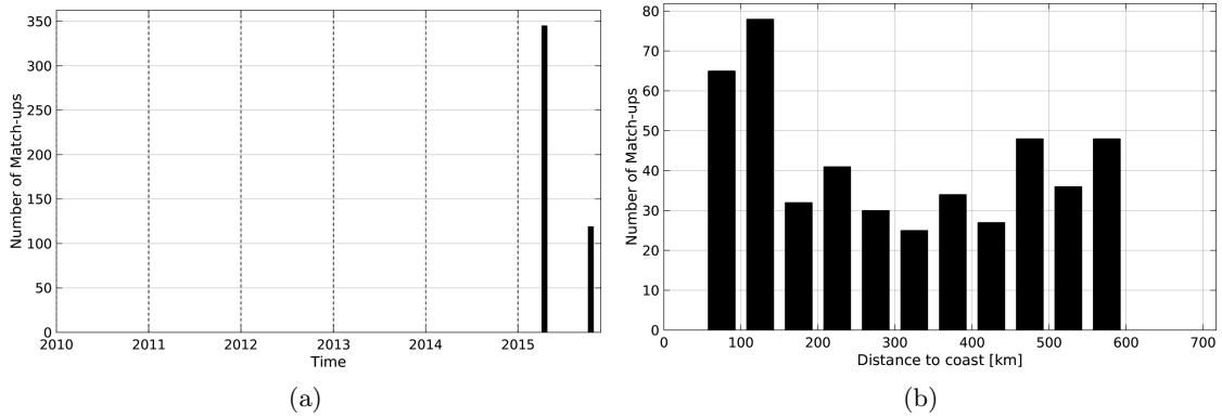
Figure 1: Number of match-ups between TSG-LEGOS-DM and SMAP-L3-RSS-V2-MONTHLY-70KM SSS as a function of time (a) and as function of the distance to coast (b) over the Bay of Bengal Pi-MEP region and for the full satellite product period.
