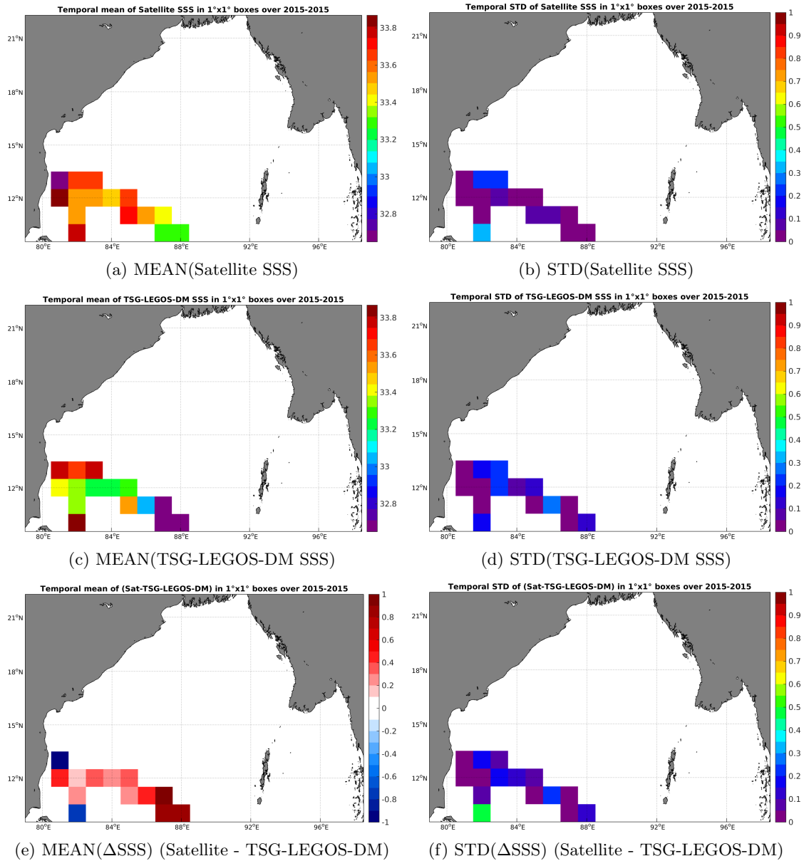
Figure 6: Temporal mean (left) and STD (right) of SSS from SMAP-L3-RSS-V2-MONTHLY-70KM (top), TSG-LEGOS-DM (middle), and of \Delta SSS (Satellite - TSG-LEGOS-DM). Only match-up pairs are used to generate these maps.
