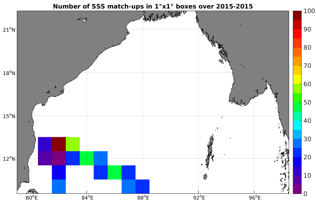
Figure 4: Number of SSS match-ups between TSG-LEGOS-DM SSS and the SMAP-L3-RSS-V2-MONTHLY-70KM SSS product for the Bay of Bengal Pi-MEP region over 1°x1° boxes and for the full satellite product period.
