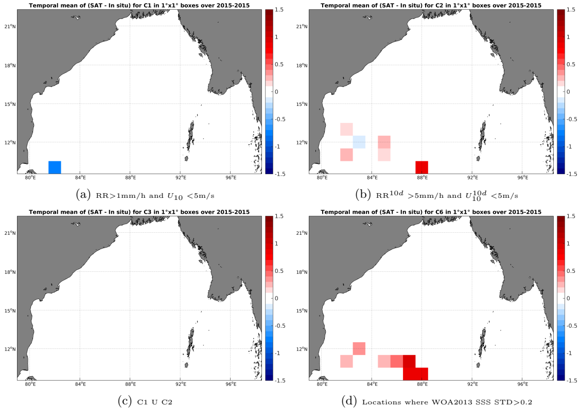
Figure 12: Temporal mean gridded over spatial boxes of size 1°x1° of \Delta SSS (SMAP-L3-RSS-V2-MONTHLY-70KM - TSG-LEGOS-DM) for 4 different subdatasets corresponding to:RR>1mm/h and U_{10} < 5m/s (a), RR^{10d} > 5mm/h and U_{10}^{10d} < 5m/s (b), C1 U C2 (c),Locations where WOA2013 SSS STD>0.2 (d).
