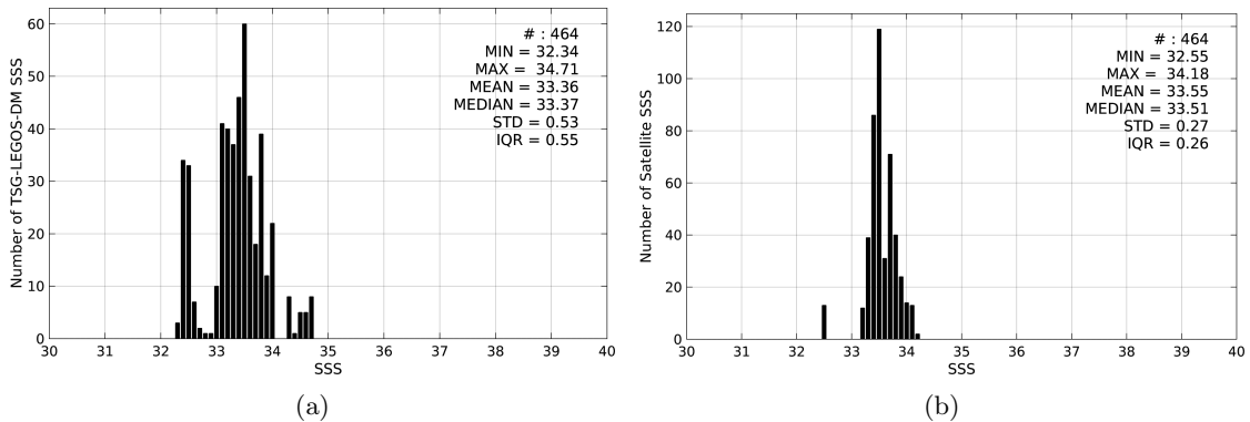
Figure 2: Histograms of SSS from TSG-LEGOS-DM (a) and SMAP-L3-RSS-V2-MONTHLY-70KM (b) considering all match-up pairs per bins of 0.1 over the Bay of Bengal Pi-MEP region and for the full satellite product period.
