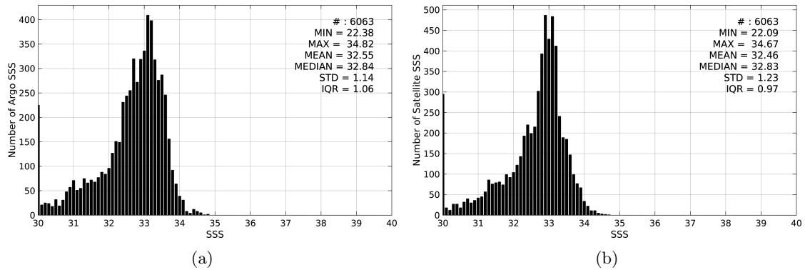
Figure 2: Histograms of SSS from Argo (a) and SMAP-L3-RSS-V2-MONTHLY-70KM (b) considering all match-up pairs per bins of 0.1 over the Bay of Bengal Pi-MEP region and for the full satellite product period.
