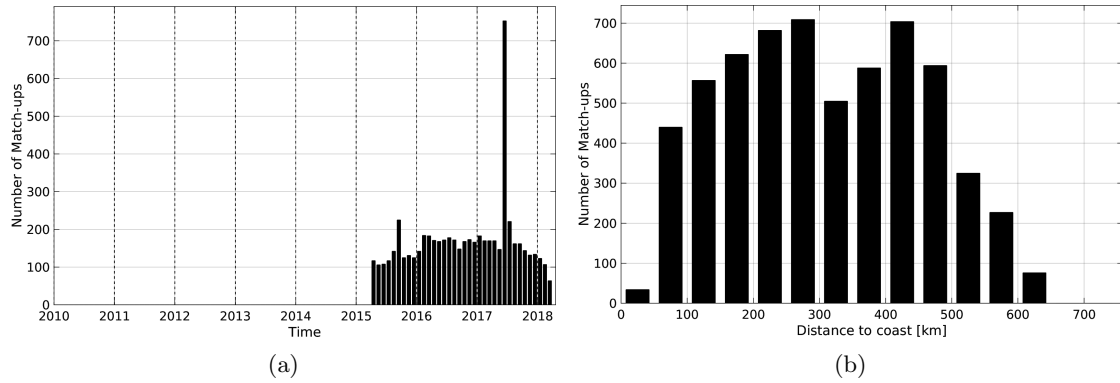
Figure 1: Number of match-ups between Argo and SMAP-L3-RSS-V2-MONTHLY-70KM SSS as a function of time (a) and as function of the distance to coast (b) over the Bay of Bengal Pi-MEP region and for the full satellite product period.
