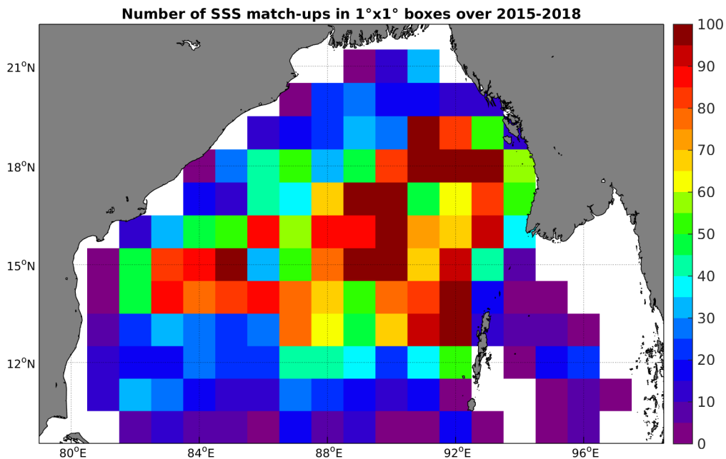
Figure 4: Number of SSS match-ups between Argo SSS and the SMAP-L3-RSS-V2-MONTHLY-70KM SSS product for the Bay of Bengal Pi-MEP region over 1°x1° boxes and for the full satellite product period.
