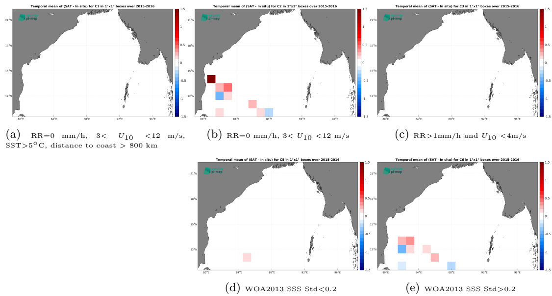
Figure 14: Temporal mean gridded over spatial boxes of size 1^\circ \times 1^\circ of \Delta\text{SSS} (SMAP SSS L3 v5.0 - 8-Day running (JPL) - TSG (LEGOS-DM)) for 5 different subdatasets corresponding to:RR=0 mm/h, 3 < U_{10} < 12 m/s, SST >5^\circ\text{C} , distance to coast > 800 km (a), RR=0 mm/h, 3 < U_{10} < 12 m/s (b), RR >1 mm/h and U_{10} < 4 m/s (c), WOA2013 SSS Std <0.2 (d), WOA2013 SSS Std >0.2 (e).
