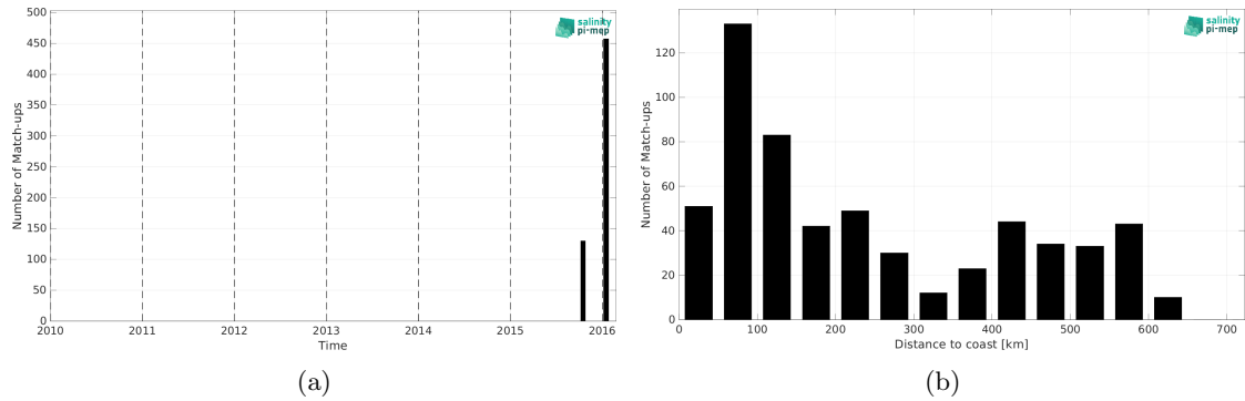
Figure 2: Number of match-ups between TSG (LEGOS-DM) and SMAP SSS L3 v5.0 - 8-Day running (JPL) SSS as a function of time (a) and as function of the distance to coast (b) over the Bay of Bengal Pi-MEP region and for the full satellite product period.
