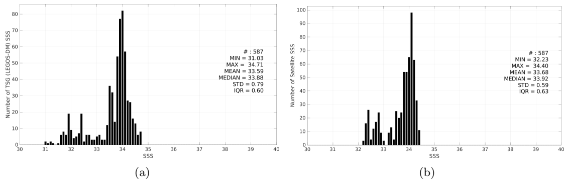
Figure 3: Histograms of SSS from TSG (LEGOS-DM) (a) and SMAP SSS L3 v5.0 - 8-Day running (JPL) (b) considering all match-up pairs per bins of 0.1 over the Bay of Bengal Pi-MEP region and for the full satellite product period.
