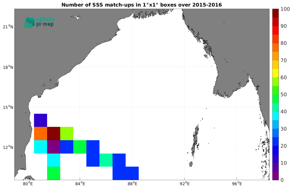
Figure 4: Number of SSS match-ups between TSG (LEGOS-DM) SSS and the SMAP SSS L3 v5.0 - 8-Day running (JPL) SSS product for the Bay of Bengal Pi-MEP region over 1^\circ \times 1^\circ boxes and for the full satellite product period.
