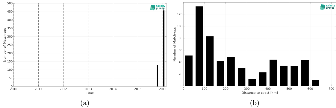
Figure 1: Number of match-ups between TSG (LEGOS-DM) and SMAP SSS L3 v5.0 - 8-Day running (JPL) SSS as a function of time (a) and as function of the distance to coast (b) over the Bay of Bengal Pi-MEP region and for the full satellite product period.
