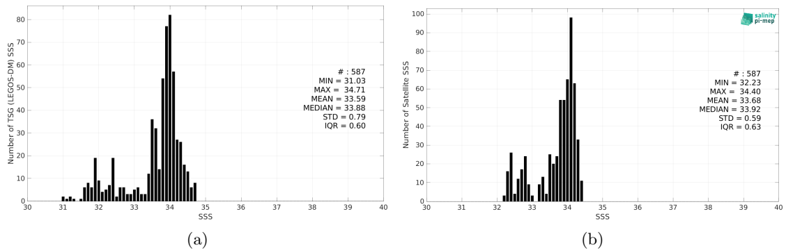
Figure 2: Histograms of SSS from TSG (LEGOS-DM) (a) and SMAP SSS L3 v5.0 - 8-Day running (JPL) (b) considering all match-up pairs per bins of 0.1 over the Bay of Bengal Pi-MEP region and for the full satellite product period.
