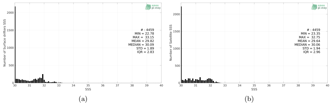
Figure 2: Histograms of SSS from Surface drifters (a) and SMAP SSS L3 v5.0 - 8-Day running (JPL) (b) considering all match-up pairs per bins of 0.1 over the Bay of Bengal Pi-MEP region and for the full satellite product period.
