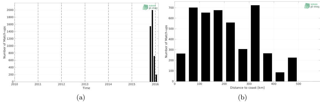
Figure 1: Number of match-ups between Surface drifters and SMAP SSS L3 v5.0 - 8-Day running (JPL) SSS as a function of time (a) and as function of the distance to coast (b) over the Bay of Bengal Pi-MEP region and for the full satellite product period.
