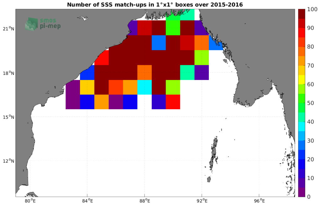
Figure 3: Number of SSS match-ups between Surface drifters SSS and the SMAP SSS L3 v5.0 - 8-Day running (JPL) SSS product for the Bay of Bengal Pi-MEP region over 1^\circ \times 1^\circ boxes and for the full satellite product period.
