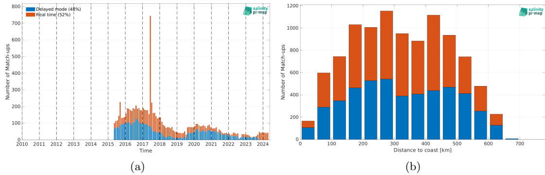
Figure 2: Number of match-ups between Argo and SMAP SSS L3 v5.0 - 8-Day running (JPL) SSS as a function of time (a) and as function of the distance to coast (b) over the Bay of Bengal Pi-MEP region and for the full satellite product period.
