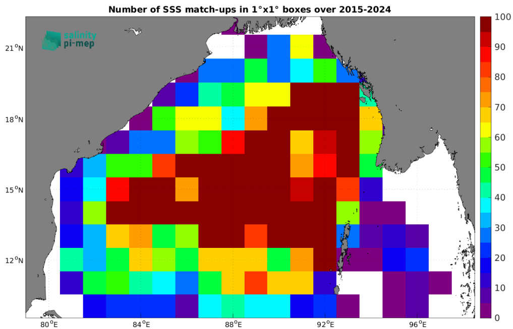
Figure 5: Number of SSS match-ups between Argo SSS and the SMAP SSS L3 v5.0 - 8-Day running (JPL) SSS product for the Bay of Bengal Pi-MEP region over 1^\circ \times 1^\circ boxes and for the full satellite product period.
