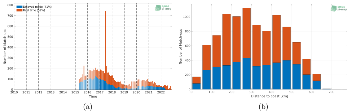
Figure 1: Number of match-ups between Argo and SMAP SSS L3 v5.0 - 8-Day running (JPL) SSS as a function of time (a) and as function of the distance to coast (b) over the Bay of Bengal Pi-MEP region and for the full satellite product period.
