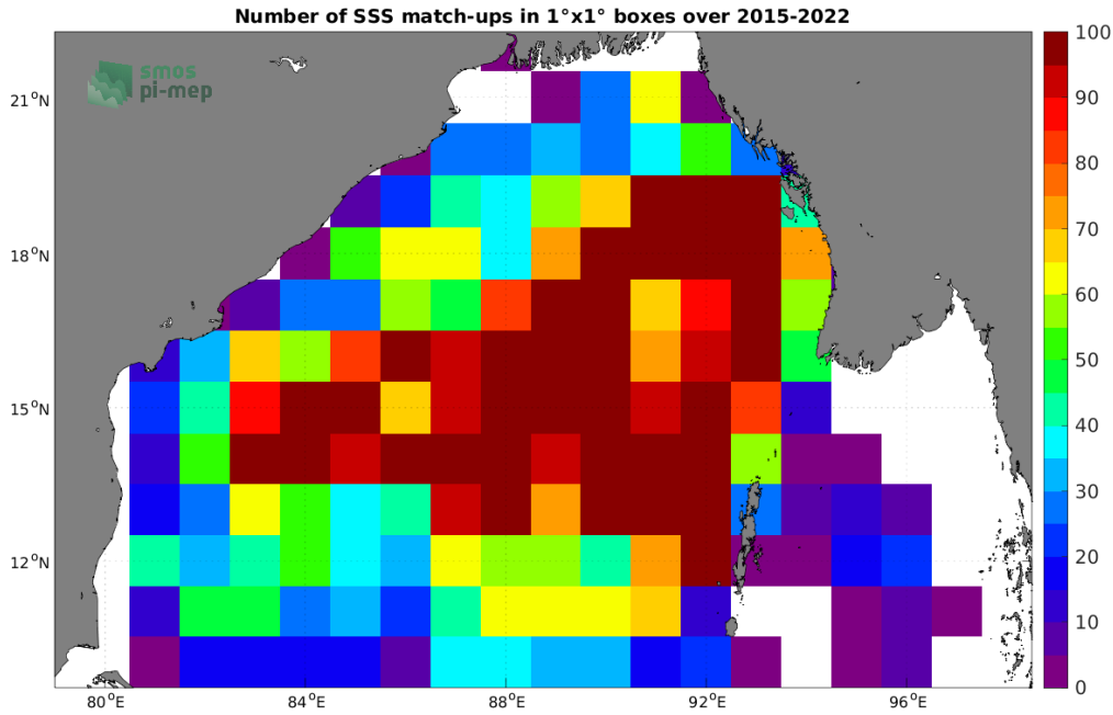
Figure 4: Number of SSS match-ups between Argo SSS and the SMAP SSS L3 v5.0 - 8-Day running (JPL) SSS product for the Bay of Bengal Pi-MEP region over 1^\circ \times 1^\circ boxes and for the full satellite product period.
