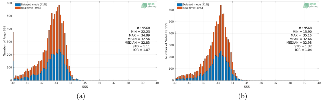
Figure 2: Histograms of SSS from Argo (a) and SMAP SSS L3 v5.0 - 8-Day running (JPL) (b) considering all match-up pairs per bins of 0.1 over the Bay of Bengal Pi-MEP region and for the full satellite product period.
