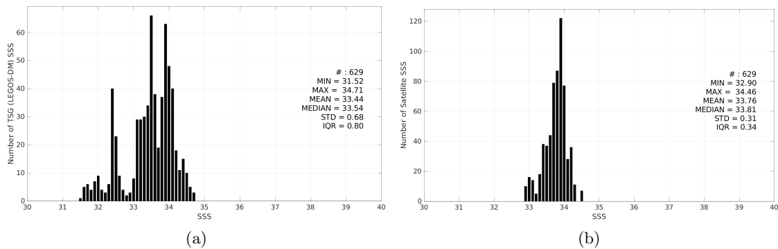
Figure 3: Histograms of SSS from TSG (LEGOS-DM) (a) and SMAP SSS L3 v5.0 - Monthly (JPL) (b) considering all match-up pairs per bins of 0.1 over the Bay of Bengal Pi-MEP region and for the full satellite product period.
