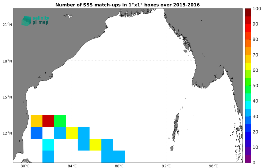
Figure 5: Number of SSS match-ups between TSG (LEGOS-DM) SSS and the SMAP SSS L3 v5.0 - Monthly (JPL) SSS product for the Bay of Bengal Pi-MEP region over 1^\circ \times 1^\circ boxes and for the full satellite product period.
