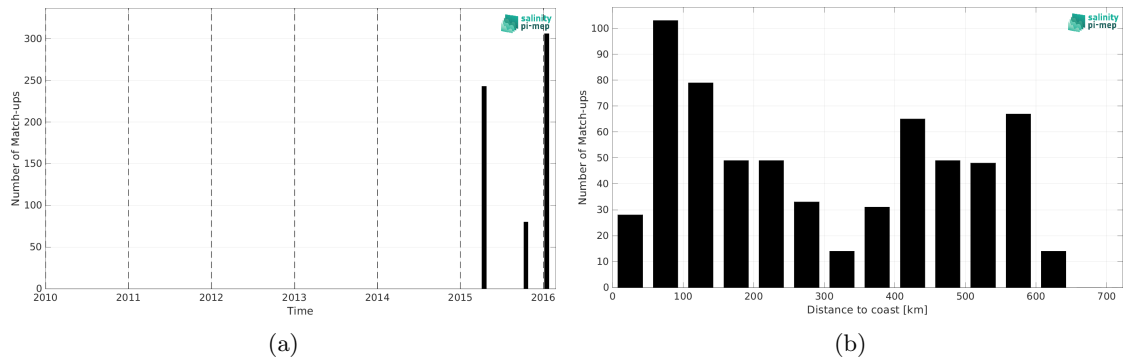
Figure 2: Number of match-ups between TSG (LEGOS-DM) and SMAP SSS L3 v5.0 - Monthly (JPL) SSS as a function of time (a) and as function of the distance to coast (b) over the Bay of Bengal Pi-MEP region and for the full satellite product period.
