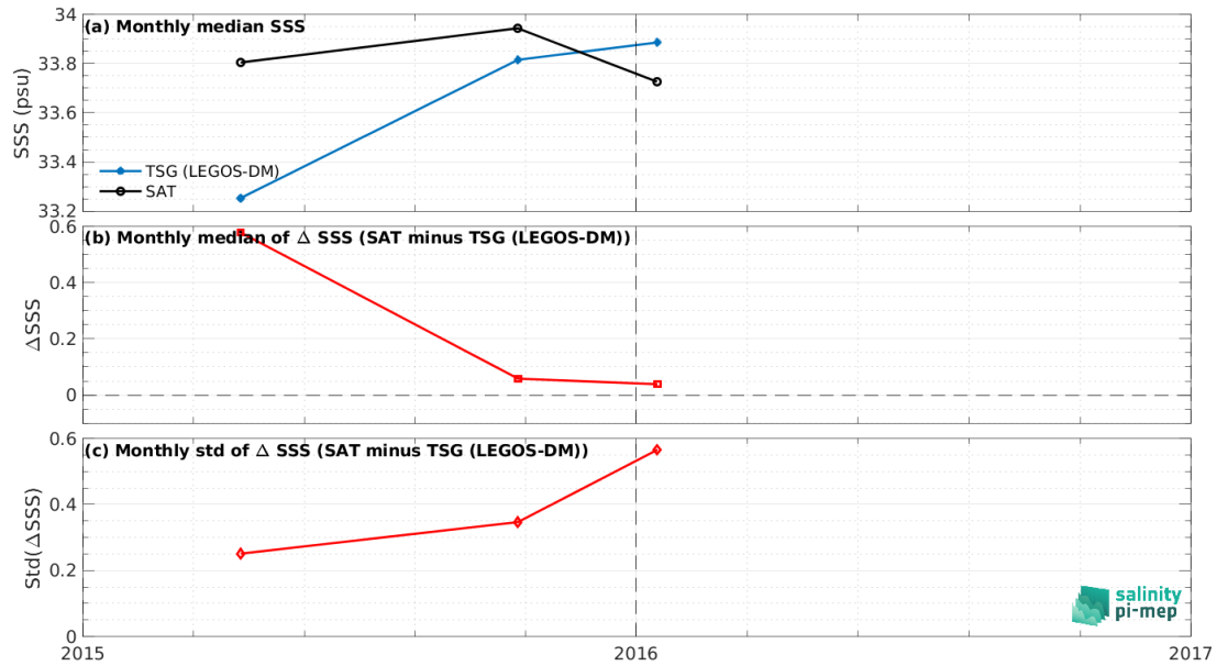
Figure 8: Time series of the monthly median SSS (top), median of \Delta SSS (Satellite - TSG (LEGOS-DM)) and Std of \Delta SSS (Satellite - TSG (LEGOS-DM)) over the Bay of Bengal Pi-MEP region considering all match-ups collected by the Pi-MEP.
