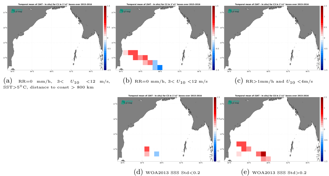
Figure 14: Temporal mean gridded over spatial boxes of size 1^\circ \times 1^\circ of \Delta SSS (SMAP SSS L3 v5.0 - Monthly (JPL) - TSG (LEGOS-DM)) for 5 different subdatasets corresponding to:RR=0 mm/h, 3 < U_{10} < 12 m/s, SST>5°C, distance to coast > 800 km (a), RR=0 mm/h, 3 < U_{10} < 12 m/s (b), RR>1mm/h and U_{10} < 4 m/s (c), WOA2013 SSS Std<0.2 (d), WOA2013 SSS Std>0.2 (e).
