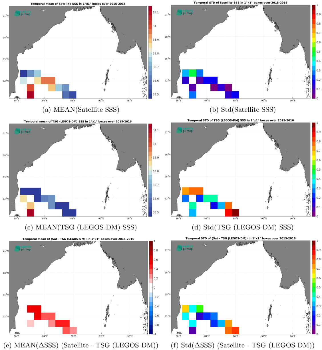
Figure 7: Temporal mean (left) and Std (right) of SSS from SMAP SSS L3 v5.0 - Monthly (JPL) (top), TSG (LEGOS-DM) (middle), and of \Delta SSS (Satellite - TSG (LEGOS-DM)). Only match-up pairs are used to generate these maps.
