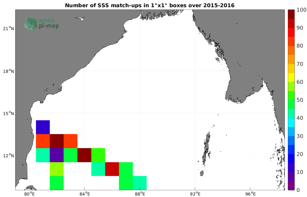
Figure 4: Number of SSS match-ups between TSG (LEGOS-DM) SSS and the SMAP SSS L3 v5.0 - Monthly (JPL) SSS product for the Bay of Bengal Pi-MEP region over 1^\circ \times 1^\circ boxes and for the full satellite product period.
