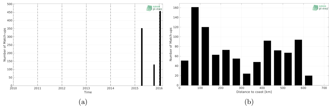
Figure 1: Number of match-ups between TSG (LEGOS-DM) and SMAP SSS L3 v5.0 - Monthly (JPL) SSS as a function of time (a) and as function of the distance to coast (b) over the Bay of Bengal Pi-MEP region and for the full satellite product period.
