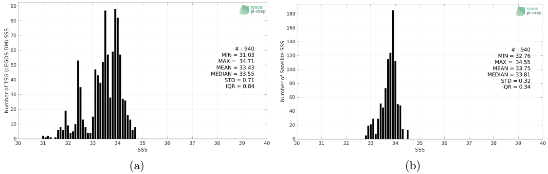
Figure 2: Histograms of SSS from TSG (LEGOS-DM) (a) and SMAP SSS L3 v5.0 - Monthly (JPL) (b) considering all match-up pairs per bins of 0.1 over the Bay of Bengal Pi-MEP region and for the full satellite product period.
