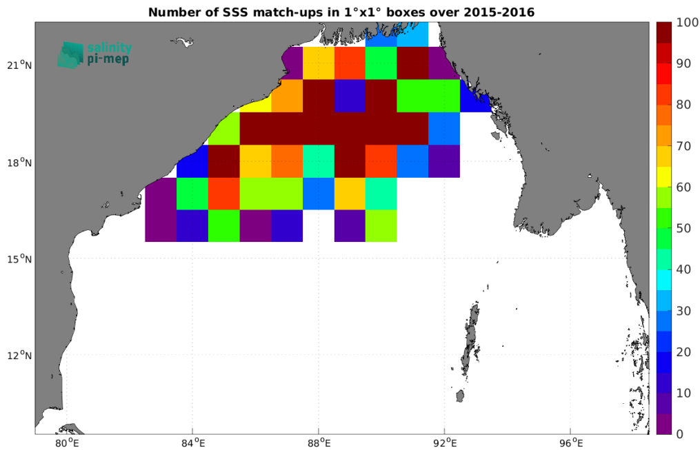
Figure 4: Number of SSS match-ups between Surface drifters SSS and the SMAP SSS L3 v5.0 - Monthly (JPL) SSS product for the Bay of Bengal Pi-MEP region over 1°×1° boxes and for the full satellite product period.
