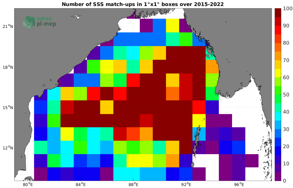
Figure 4: Number of SSS match-ups between Argo SSS and the SMAP SSS L3 v5.0 - Monthly (JPL) SSS product for the Bay of Bengal Pi-MEP region over 1^{\circ} \times 1^{\circ} boxes and for the full satellite product period.
