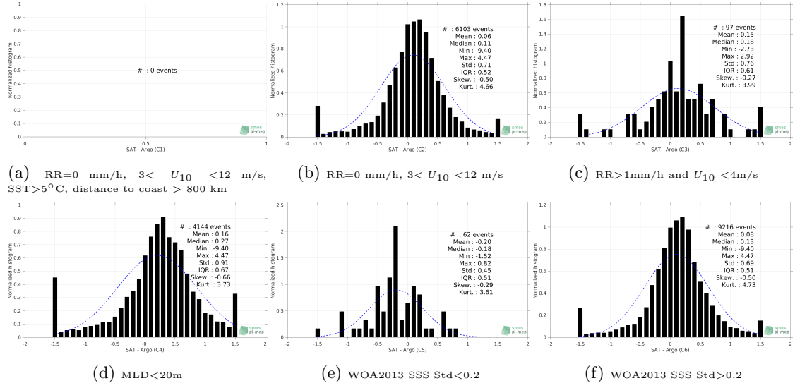
Figure 13: Normalized histogram of \Delta SSS (SMAP SSS L3 v5.0 - Monthly (JPL) - Argo) for 6 different subdatasets corresponding to: RR=0 mm/h, 3 < U_{10} < 12 m/s, SST > 5^\circ C , distance to coast > 800 km (a), RR=0 mm/h, 3 < U_{10} < 12 m/s (b), RR > 1 mm/h and U_{10} < 4 m/s (c), MLD < 20 m (d), WOA2013 SSS Std < 0.2 (e), WOA2013 SSS Std > 0.2 (f).
