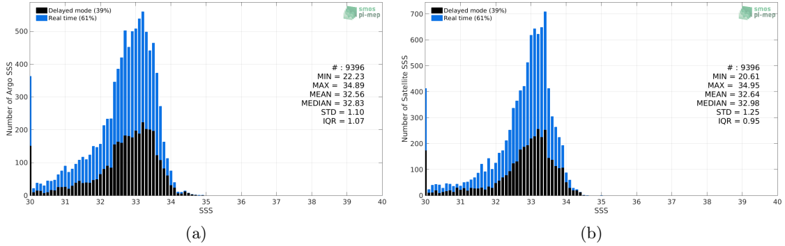
Figure 2: Histograms of SSS from Argo (a) and SMAP SSS L3 v5.0 - Monthly (JPL) (b) considering all match-up pairs per bins of 0.1 over the Bay of Bengal Pi-MEP region and for the full satellite product period.
