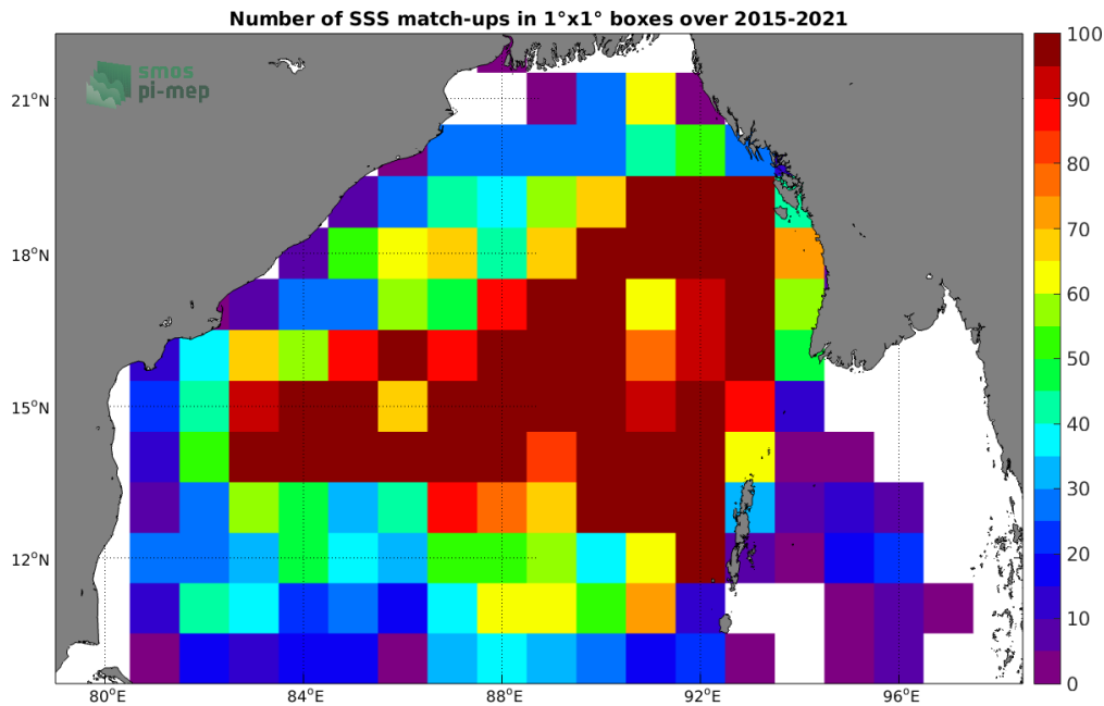
Figure 4: Number of SSS match-ups between Argo SSS and the SMAP SSS L3 v5.0 - Monthly (JPL) SSS product for the Bay of Bengal Pi-MEP region over 1^\circ \times 1^\circ boxes and for the full satellite product period.
