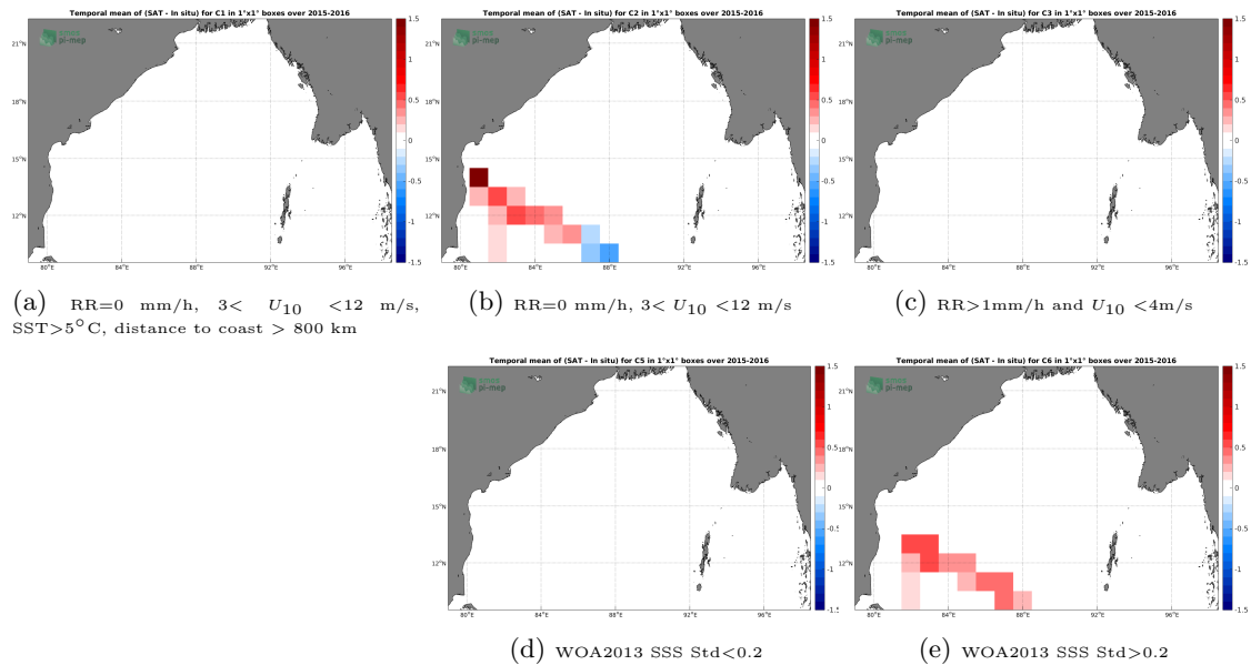
Figure 12: Temporal mean gridded over spatial boxes of size 1^\circ \times 1^\circ of \Delta SSS (SMAP-L3-JPL-V4.2-MONTHLY-60KM - TSG-LEGOS-DM) for 5 different subdatasets corresponding to:RR=0 mm/h, 3 < U_{10} < 12 m/s, SST >5^\circ C, distance to coast > 800 km (a), RR=0 mm/h, 3 < U_{10} < 12 m/s (b), RR >1 mm/h and U_{10} < 4 m/s (c), WOA2013 SSS Std <0.2 (d), WOA2013 SSS Std >0.2 (e).
