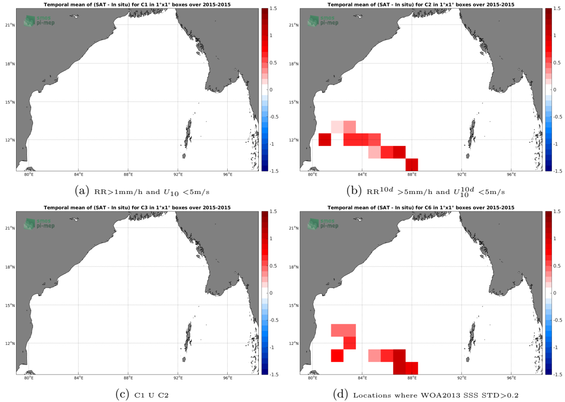
Figure 12: Temporal mean gridded over spatial boxes of size 1^\circ \times 1^\circ of \Delta SSS (SMAP-L3-JPL-V4-8DAY-RUNNING-60KM - TSG-LEGOS-DM) for 4 different subdatasets corresponding to: RR > 1mm/h and U_{10} < 5\text{m/s} (a), RR^{10d} > 5\text{mm/h} and U_{10}^{10d} < 5\text{m/s} (b), C1 U C2 (c), Locations where WOA2013 SSS STD > 0.2 (d).
