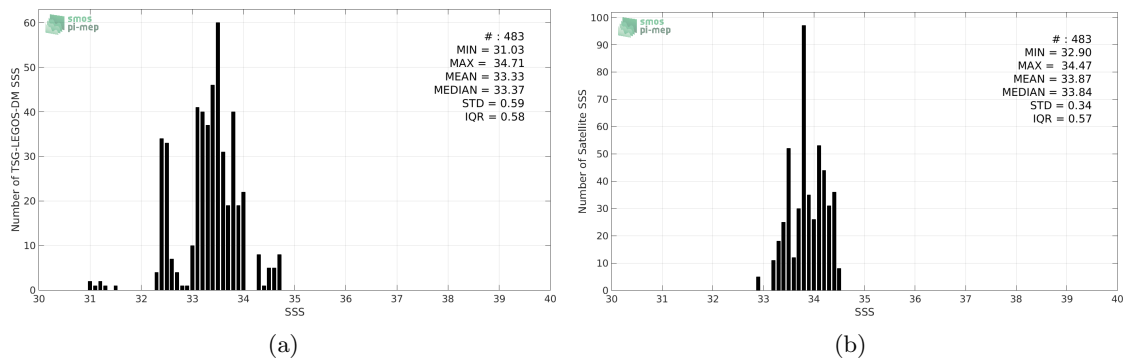
Figure 2: Histograms of SSS from TSG-LEGOS-DM (a) and SMAP-L3-JPL-V4-8DAY-RUNNING-60KM (b) considering all match-up pairs per bins of 0.1 over the Bay of Bengal Pi-MEP region and for the full satellite product period.
