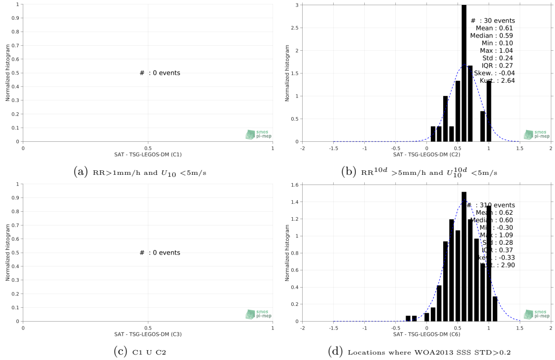
Figure 13: Normalized histogram of \Delta\text{SSS} (SMAP-L3-JPL-V4-8DAY-RUNNING-60KM - TSG-LEGOS-DM) for 6 different subdatasets corresponding to: RR > 1\text{mm/h} and U_{10} < 5\text{m/s} (a), RR^{10d} > 5\text{mm/h} and U_{10}^{10d} < 5\text{m/s} (b), C1 \cup C2 (c), Locations where WOA2013 SSS STD > 0.2 (d).
