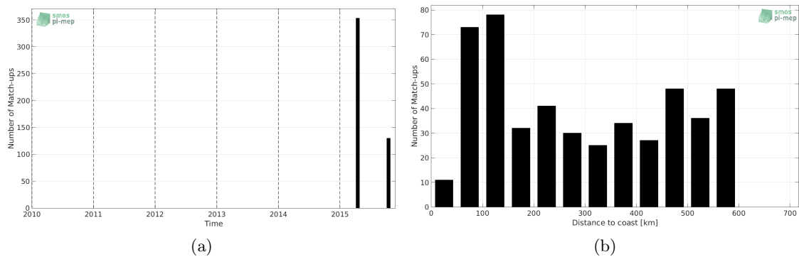
Figure 1: Number of match-ups between TSG-LEGOS-DM and SMAP-L3-JPL-V4-8DAY-RUNNING-60KM SSS as a function of time (a) and as function of the distance to coast (b) over the Bay of Bengal Pi-MEP region and for the full satellite product period.
