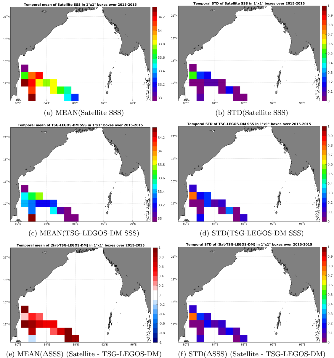
Figure 6: Temporal mean (left) and STD (right) of SSS from SMAP-L3-JPL-V4-8DAY-RUNNING-60KM (top), TSG-LEGOS-DM (middle), and of \Delta SSS (Satellite - TSG-LEGOS-DM). Only match-up pairs are used to generate these maps.
