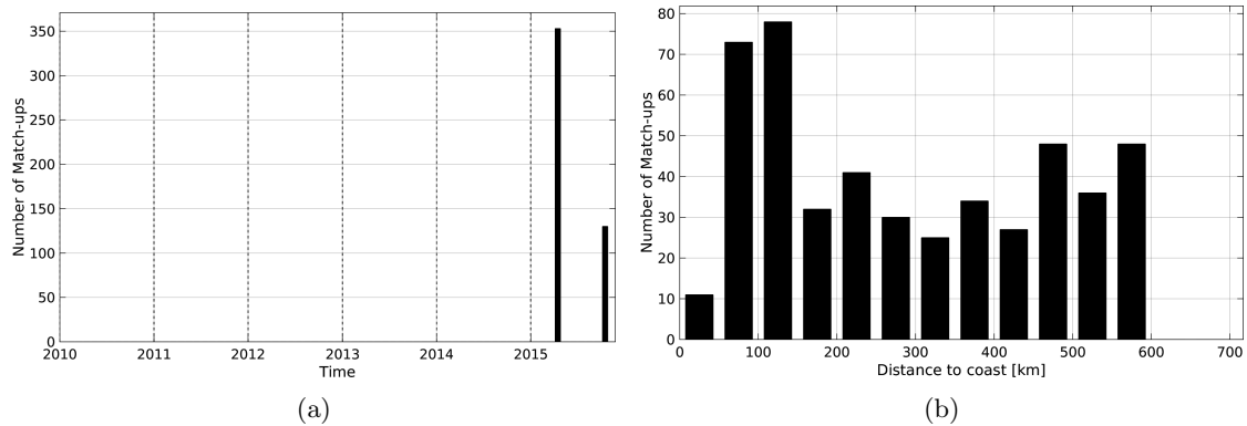
Figure 1: Number of match-ups between TSG-LEGOS-DM and SMAP-L3-JPL-V4-8DAY-RUNNING-60KM SSS as a function of time (a) and as function of the distance to coast (b) over the Bay of Bengal Pi-MEP region and for the full satellite product period.
