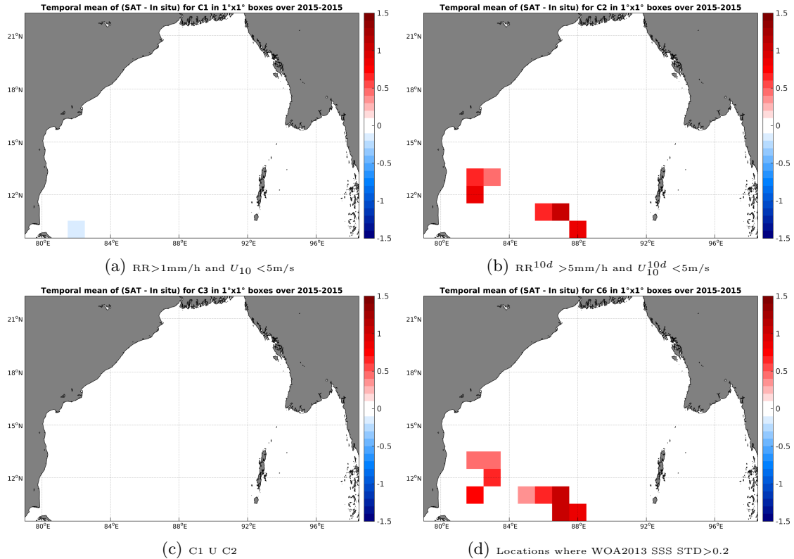
Figure 12: Temporal mean gridded over spatial boxes of size 1^\circ \times 1^\circ of \Delta SSS (SMAP-L3-JPL-V4-8DAY-RUNNING-60KM - TSG-LEGOS-DM) for 4 different subdatasets corresponding to: RR > 1 mm/h and U_{10} < 5 m/s (a), RR^{10d} > 5 mm/h and U_{10}^{10d} < 5 m/s (b), C1 U C2 (c), Locations where WOA2013 SSS STD > 0.2 (d).
