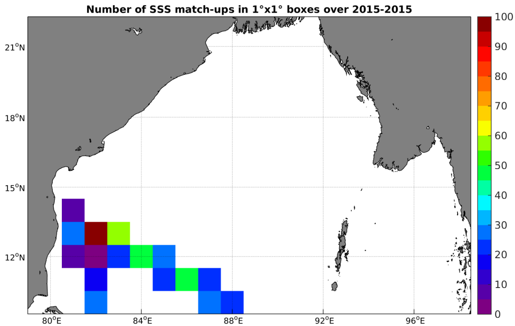
Figure 4: Number of SSS match-ups between TSG-LEGOS-DM SSS and the SMAP-L3-JPL-V4-8DAY-RUNNING-60KM SSS product for the Bay of Bengal Pi-MEP region over 1^\circ \times 1^\circ boxes and for the full satellite product period.
