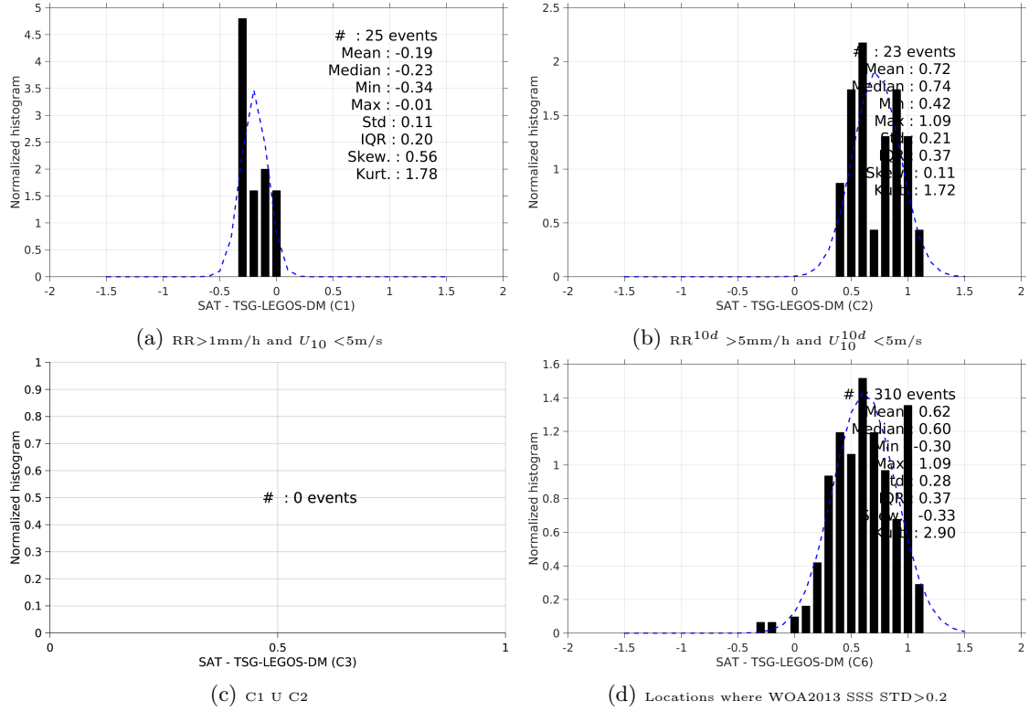
Figure 13: Normalized histogram of \Delta\text{SSS} (SMAP-L3-JPL-V4-8DAY-RUNNING-60KM - TSG-LEGOS-DM) for 6 different subdatasets corresponding to: RR>1mm/h and U_{10} < 5\text{m/s} (a), RR^{10d} > 5\text{mm/h} and U_{10}^{10d} < 5\text{m/s} (b), C1 U C2 (c), Locations where WOA2013 SSS STD>0.2 (d).
