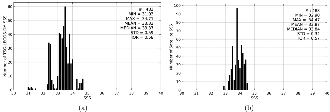
Figure 2: Histograms of SSS from TSG-LEGOS-DM (a) and SMAP-L3-JPL-V4-8DAY-RUNNING-60KM (b) considering all match-up pairs per bins of 0.1 over the Bay of Bengal Pi-MEP region and for the full satellite product period.
