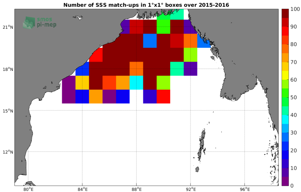
Figure 3: Number of SSS match-ups between Surface drifters SSS and the SMAP-L3-JPL-V4-8DAY-RUNNING-60KM SSS product for the Bay of Bengal Pi-MEP region over 1^{\circ} \times 1^{\circ} boxes and for the full satellite product period.
