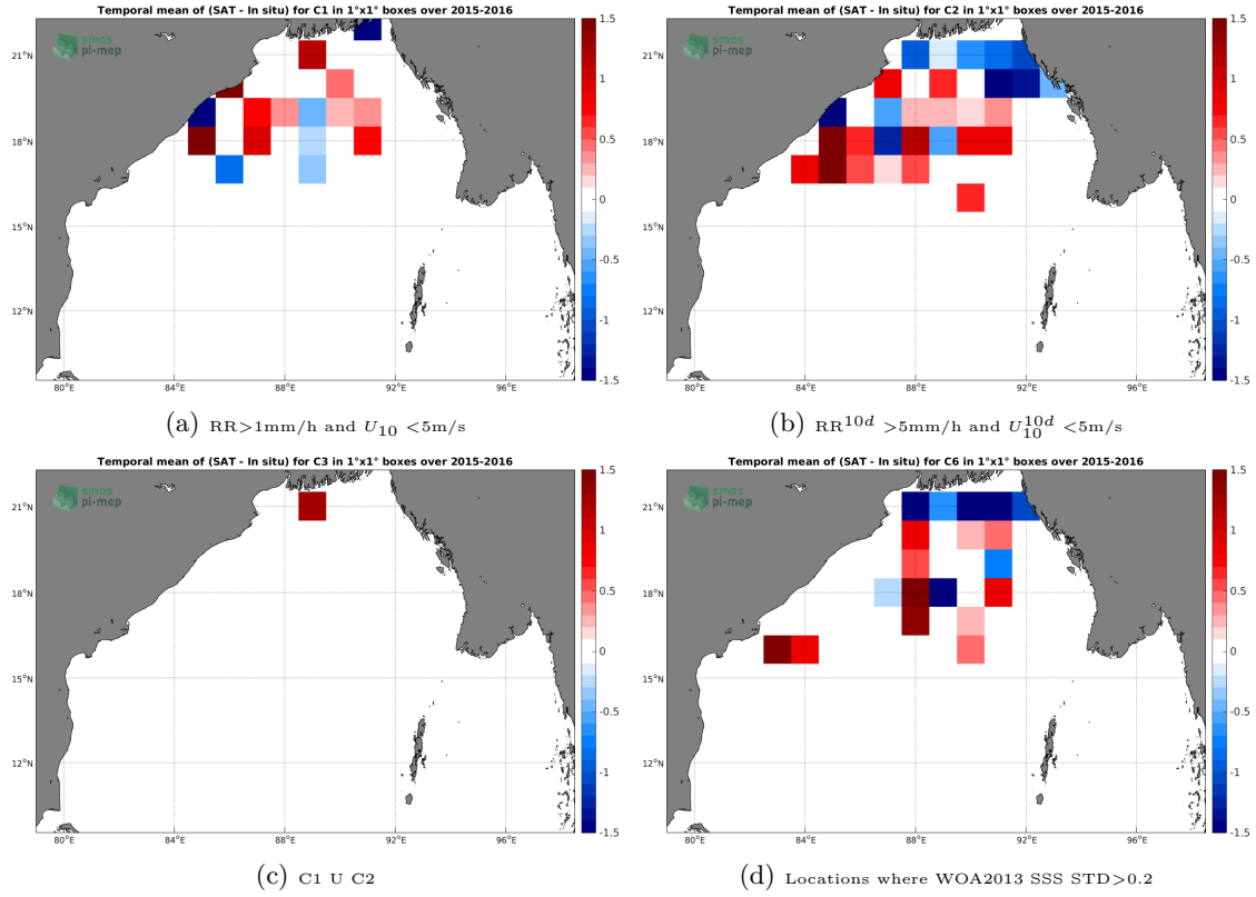
Figure 11: Temporal mean gridded over spatial boxes of size 1^\circ \times 1^\circ of \Delta SSS (SMAP-L3-JPL-V4-8DAY-RUNNING-60KM - Surface drifters) for 4 different subdatasets corresponding to: RR > 1mm/h and U_{10} < 5\text{m/s} (a), RR^{10d} > 5\text{mm/h} and U_{10}^{10d} < 5\text{m/s} (b), C1 U C2 (c), Locations where WOA2013 SSS STD > 0.2 (d).
