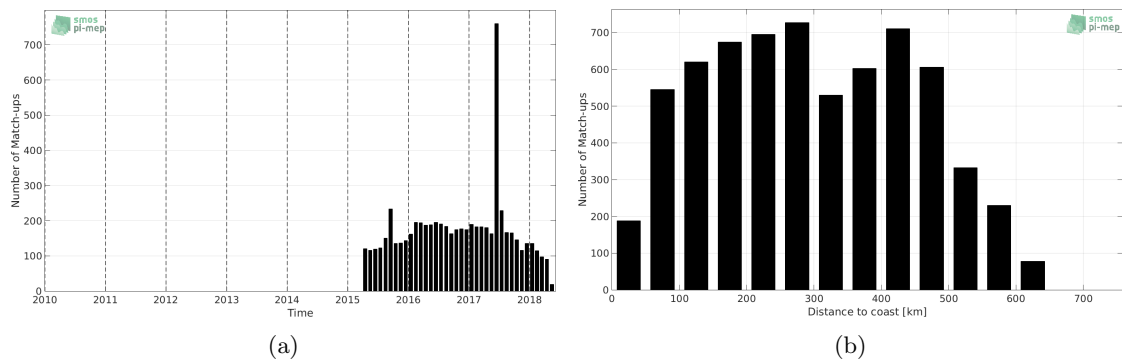
Figure 1: Number of match-ups between Argo and SMAP-L3-JPL-V4-8DAY-RUNNING-60KM SSS as a function of time (a) and as function of the distance to coast (b) over the Bay of Bengal Pi-MEP region and for the full satellite product period.
