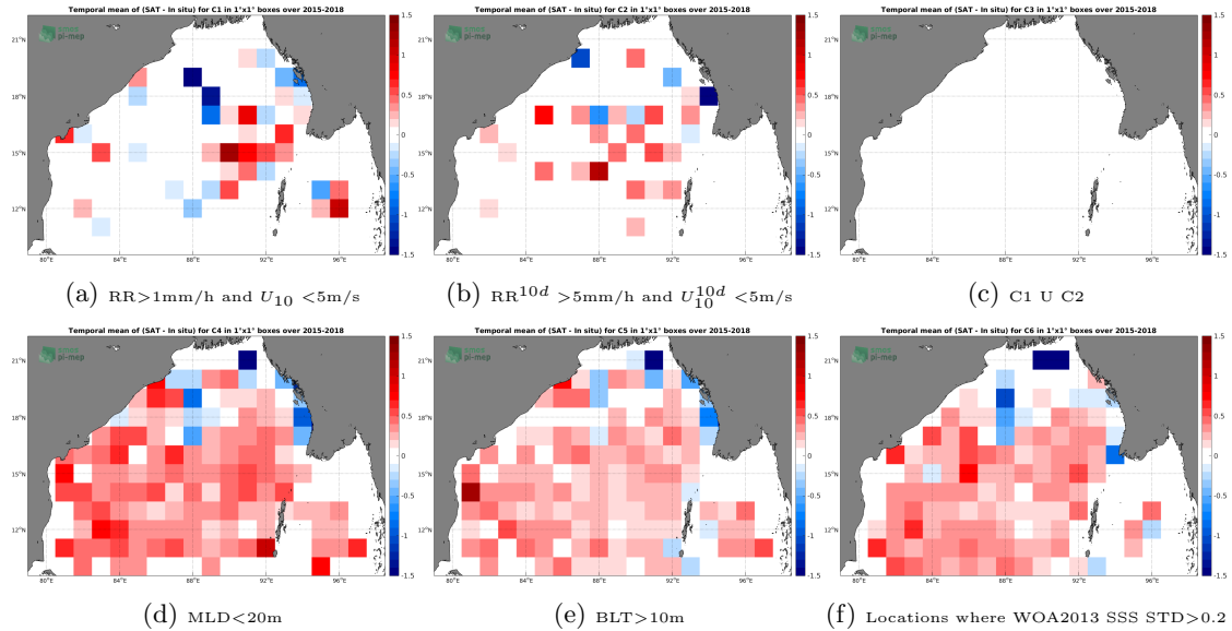
Figure 12: Temporal mean gridded over spatial boxes of size 1^\circ \times 1^\circ of \Delta\text{SSS} (SMAP-L3-JPL-V4-8DAY-RUNNING-60KM - Argo) for 6 different subdatasets corresponding to: RR > 1\text{mm/h} and U_{10} < 5\text{m/s} (a), RR^{10d} > 5\text{mm/h} and U_{10}^{10d} < 5\text{m/s} (b), C1 U C2 (c), MLD < 20\text{m} (d), BLT > 10\text{m} (e), Locations where WOA2013 SSS STD > 0.2 (f).
