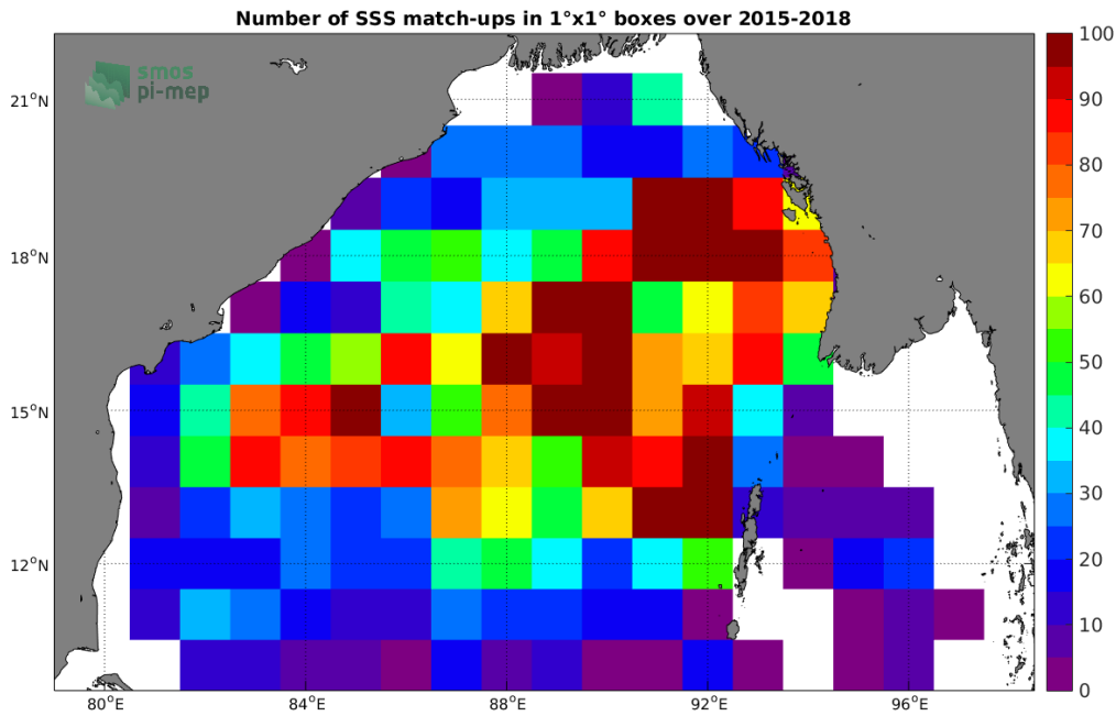
Figure 4: Number of SSS match-ups between Argos SSS and the SMAP-L3-JPL-V4-8DAY-RUNNING-60KM SSS product for the Bay of Bengal Pi-MEP region over 1^{\circ} \times 1^{\circ} boxes and for the full satellite product period.
