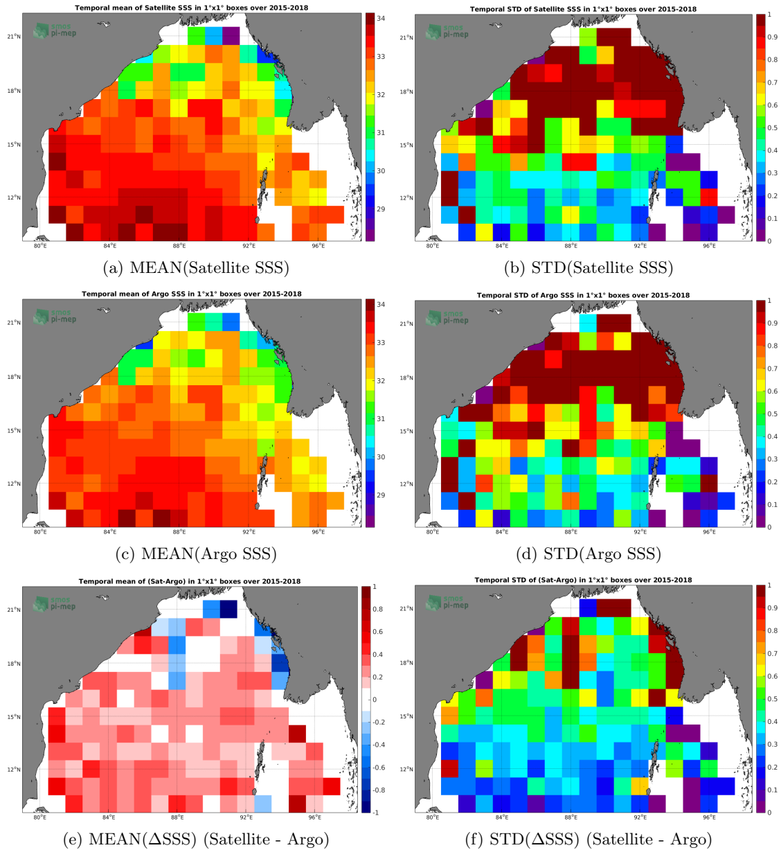
Figure 6: Temporal mean (left) and STD (right) of SSS from SMAP-L3-JPL-V4-8DAY-RUNNING-60KM (top), Argo (middle), and of \Delta SSS (Satellite - Argo). Only match-up pairs are used to generate these maps.
