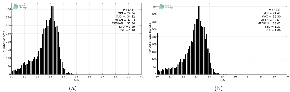
Figure 2: Histograms of SSS from Argo (a) and SMAP-L3-JPL-V4-8DAY-RUNNING-60KM (b) considering all match-up pairs per bins of 0.1 over the Bay of Bengal Pi-MEP region and for the full satellite product period.
