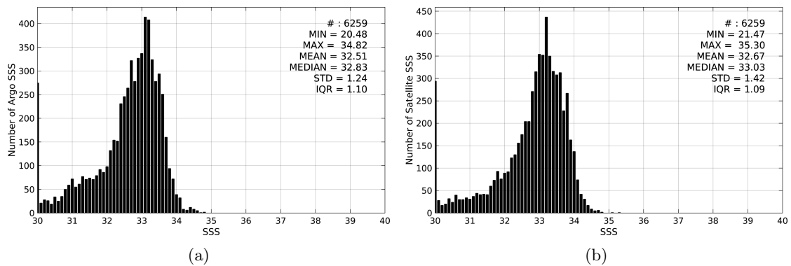
Figure 2: Histograms of SSS from Argo (a) and SMAP-L3-JPL-V4-8DAY-RUNNING-60KM (b) considering all match-up pairs per bins of 0.1 over the Bay of Bengal Pi-MEP region and for the full satellite product period.
