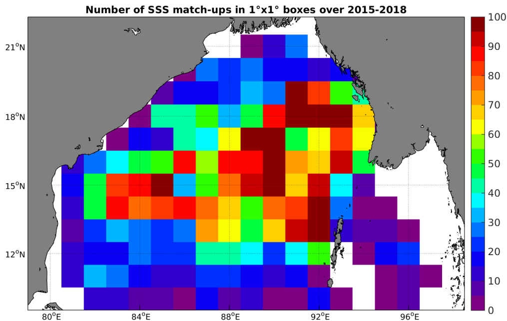
Figure 4: Number of SSS match-ups between Argo SSS and the SMAP-L3-JPL-V4-8DAY-RUNNING-60KM SSS product for the Bay of Bengal Pi-MEP region over 1°x1° boxes and for the full satellite product period.
