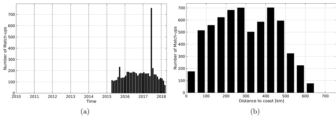
Figure 1: Number of match-ups between Argo and SMAP-L3-JPL-V4-8DAY-RUNNING-60KM SSS as a function of time (a) and as function of the distance to coast (b) over the Bay of Bengal Pi-MEP region and for the full satellite product period.
