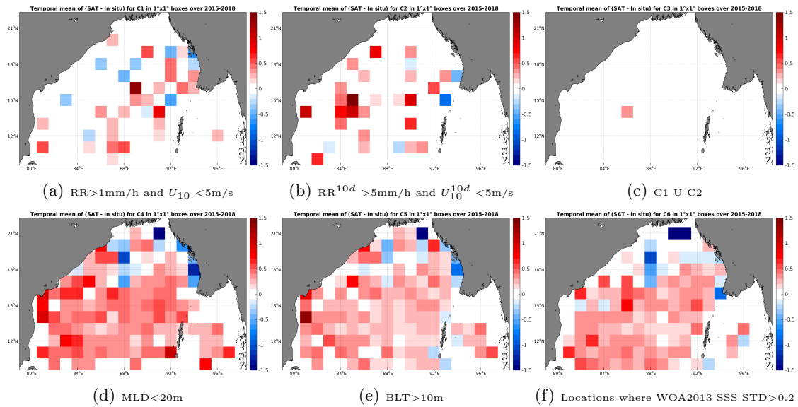
Figure 12: Temporal mean gridded over spatial boxes of size 1^\circ \times 1^\circ of \Delta SSS (SMAP-L3-JPL-V4-8DAY-RUNNING-60KM - Argo) for 6 different subdatasets corresponding to: RR > 1\text{mm/h} and U_{10} < 5\text{m/s} (a), RR^{10d} > 5\text{mm/h} and U_{10}^{10d} < 5\text{m/s} (b), C1 U C2 (c), MLD < 20\text{m} (d), BLT > 10\text{m} (e), Locations where WOA2013 SSS STD > 0.2 (f).
