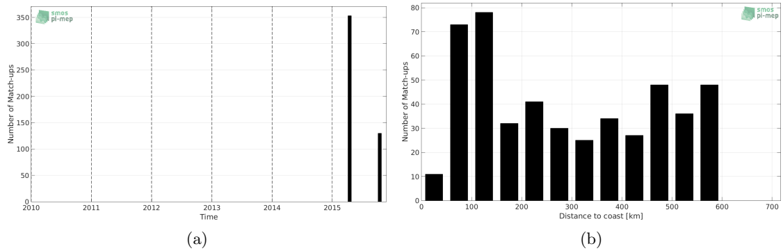
Figure 1: Number of match-ups between TSG-LEGOS-DM and SMAP-L3-JPL-V4-MONTHLY-60KM SSS as a function of time (a) and as function of the distance to coast (b) over the Bay of Bengal Pi-MEP region and for the full satellite product period.
