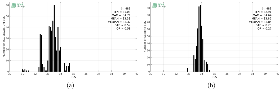
Figure 2: Histograms of SSS from TSG-LEGOS-DM (a) and SMAP-L3-JPL-V4-MONTHLY-60KM (b) considering all match-up pairs per bins of 0.1 over the Bay of Bengal Pi-MEP region and for the full satellite product period.
