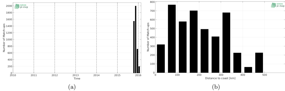
Figure 1: Number of match-ups between Surface drifters and SMAP-L3-JPL-V4-MONTHLY-60KM SSS as a function of time (a) and as function of the distance to coast (b) over the Bay of Bengal Pi-MEP region and for the full satellite product period.
