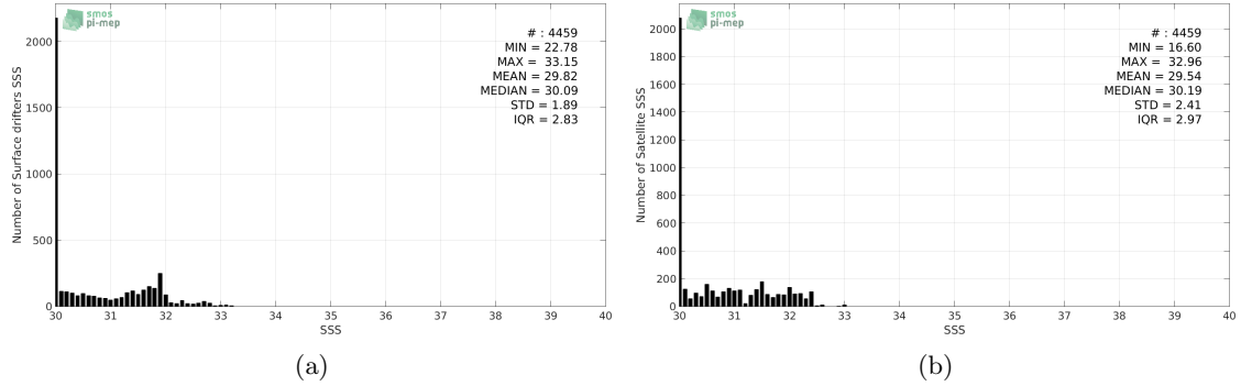
Figure 2: Histograms of SSS from Surface drifters (a) and SMAP-L3-JPL-V4-MONTHLY-60KM (b) considering all match-up pairs per bins of 0.1 over the Bay of Bengal Pi-MEP region and for the full satellite product period.
