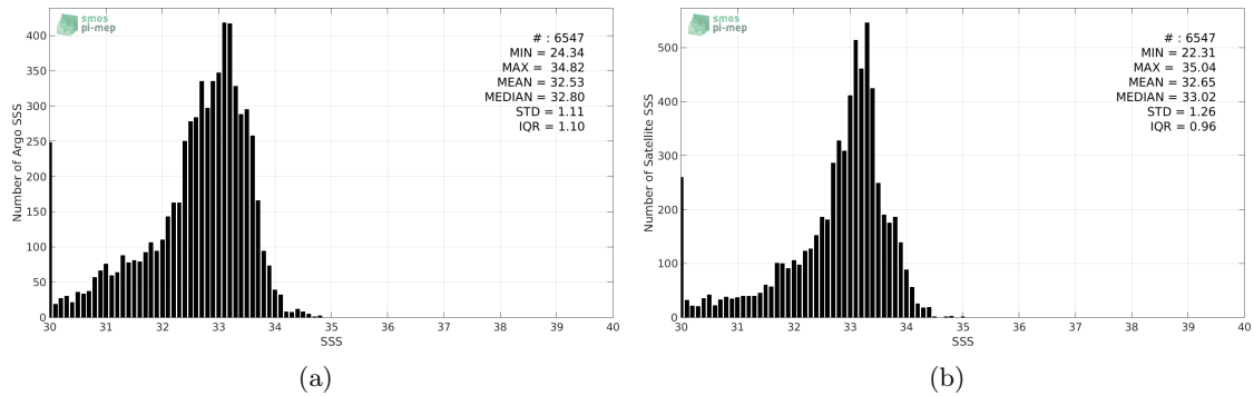
Figure 2: Histograms of SSS from Argo (a) and SMAP-L3-JPL-V4-MONTHLY-60KM (b) considering all match-up pairs per bins of 0.1 over the Bay of Bengal Pi-MEP region and for the full satellite product period.
