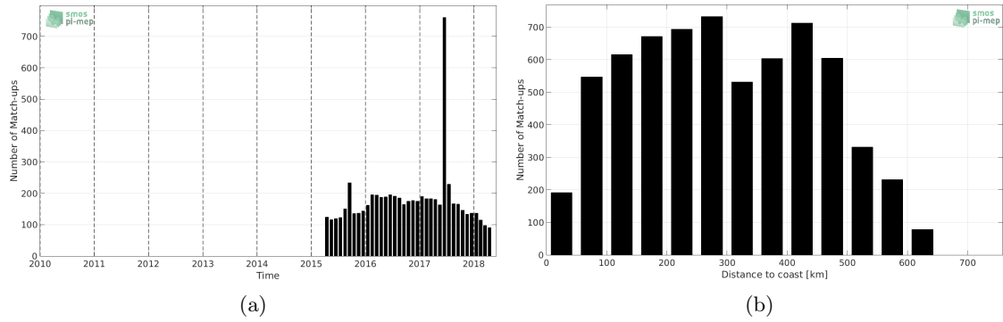
Figure 1: Number of match-ups between Argo and SMAP-L3-JPL-V4-MONTHLY-60KM SSS as a function of time (a) and as function of the distance to coast (b) over the Bay of Bengal Pi-MEP region and for the full satellite product period.
