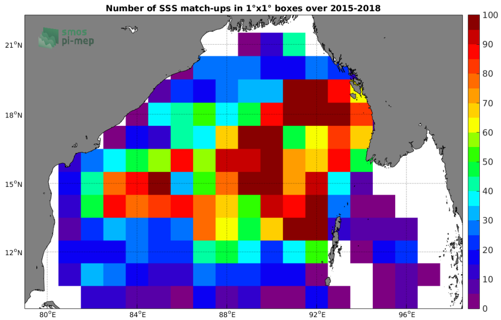
Figure 4: Number of SSS match-ups between Argo SSS and the SMAP-L3-JPL-V4-MONTHLY-60KM SSS product for the Bay of Bengal Pi-MEP region over 1^\circ \times 1^\circ boxes and for the full satellite product period.
