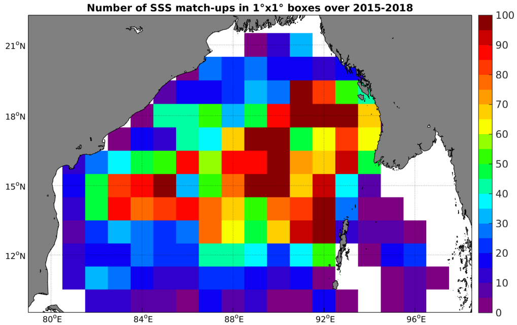
Figure 4: Number of SSS match-ups between Argo SSS and the SMAP-L3-JPL-V4-MONTHLY-60KM SSS product for the Bay of Bengal Pi-MEP region over 1°x1° boxes and for the full satellite product period.
