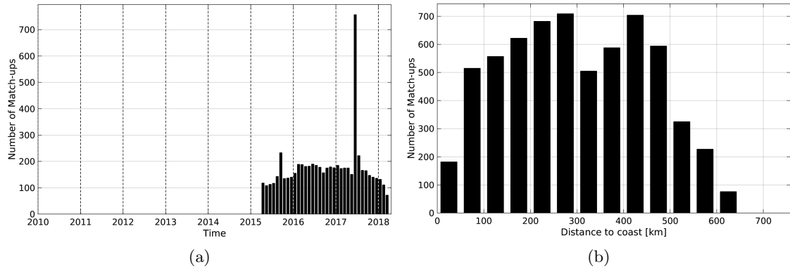
Figure 1: Number of match-ups between Argo and SMAP-L3-JPL-V4-MONTHLY-60KM SSS as a function of time (a) and as function of the distance to coast (b) over the Bay of Bengal Pi-MEP region and for the full satellite product period.
