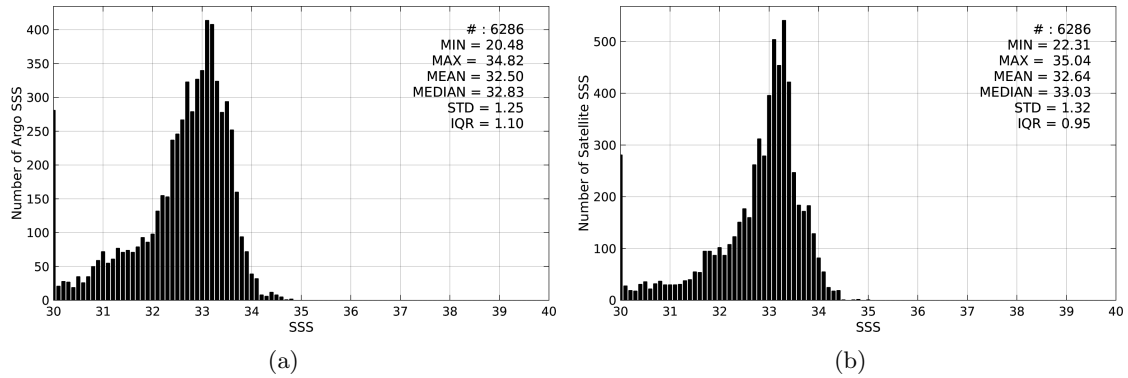
Figure 2: Histograms of SSS from Argo (a) and SMAP-L3-JPL-V4-MONTHLY-60KM (b) considering all match-up pairs per bins of 0.1 over the Bay of Bengal Pi-MEP region and for the full satellite product period.
