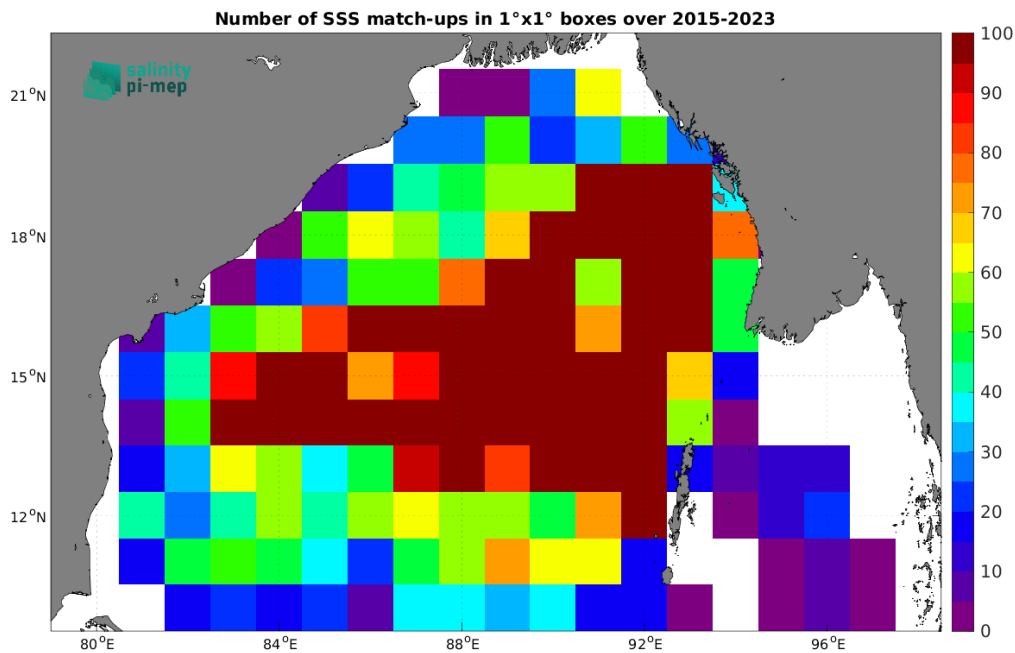
Figure 4: Number of SSS match-ups between Argo SSS and the SMAP SSS L2-AVERAGED v5 (RSS) SSS product for the Bay of Bengal Pi-MEP region over 1^\circ \times 1^\circ boxes and for the full satellite product period.
