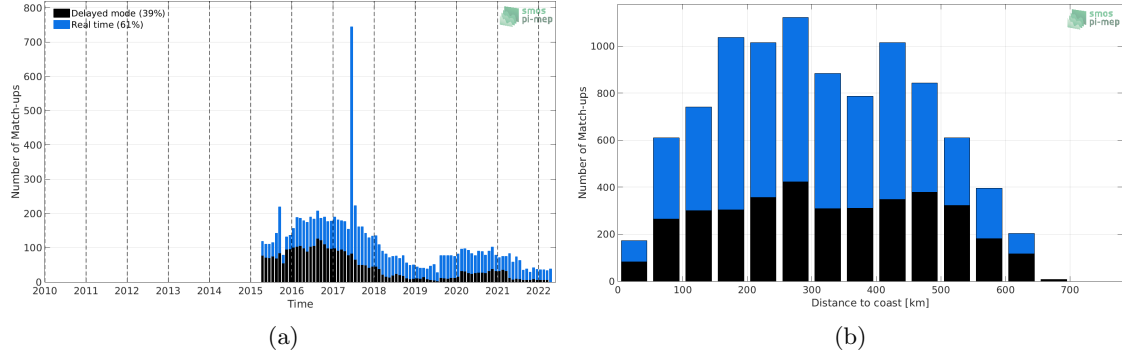
Figure 1: Number of match-ups between Argo and SMAP SSS L2-AVERAGED v5 (RSS) SSS as a function of time (a) and as function of the distance to coast (b) over the Bay of Bengal Pi-MEP region and for the full satellite product period.
