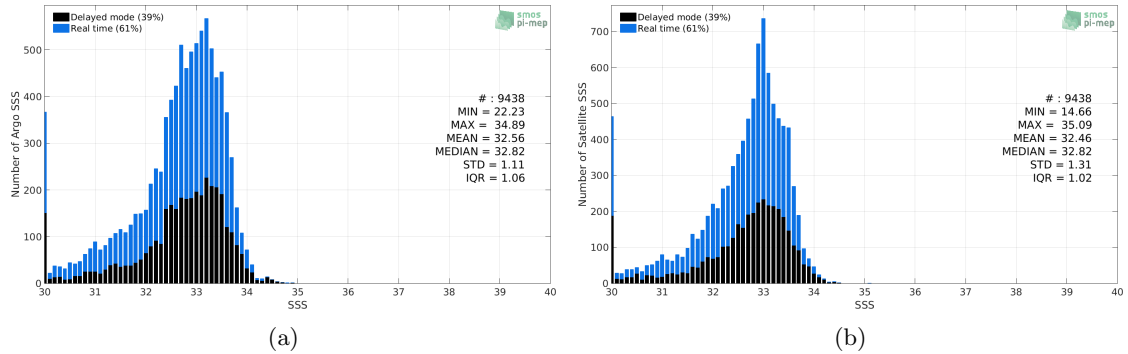
Figure 2: Histograms of SSS from Argo (a) and SMAP SSS L2-AVERAGED v5 (RSS) (b) considering all match-up pairs per bins of 0.1 over the Bay of Bengal Pi-MEP region and for the full satellite product period.
