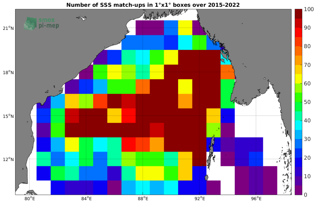
Figure 4: Number of SSS match-ups between Argo SSS and the SMAP SSS L2-AVERAGED v5 (RSS) SSS product for the Bay of Bengal Pi-MEP region over 1°×1° boxes and for the full satellite product period.
