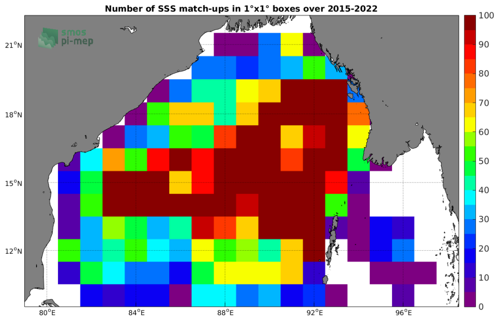
Figure 4: Number of SSS match-ups between Argo SSS and the SMAP SSS L2-AVERAGED v5.0 (JPL) SSS product for the Bay of Bengal Pi-MEP region over 1^\circ \times 1^\circ boxes and for the full satellite product period.
