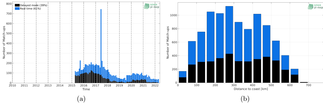
Figure 1: Number of match-ups between Argo and SMAP SSS L2-AVERAGED v5.0 (JPL) SSS as a function of time (a) and as function of the distance to coast (b) over the Bay of Bengal Pi-MEP region and for the full satellite product period.
