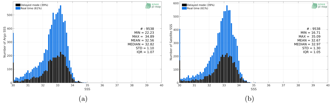
Figure 2: Histograms of SSS from Argo (a) and SMAP SSS L2-AVERAGED v5.0 (JPL) (b) considering all match-up pairs per bins of 0.1 over the Bay of Bengal Pi-MEP region and for the full satellite product period.
