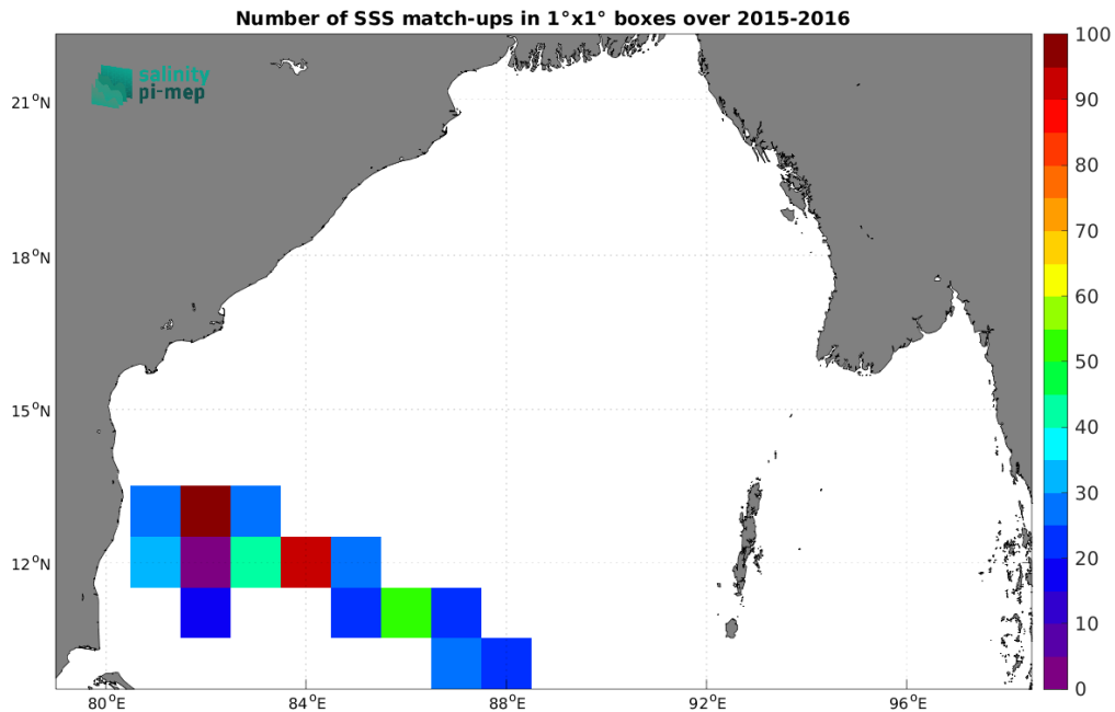
Figure 5: Number of SSS match-ups between TSG (LEGOS-DM) SSS and the SMAP SSS L2 v6 (RSS) SSS product for the Bay of Bengal Pi-MEP region over 1^\circ \times 1^\circ boxes and for the full satellite product period.
