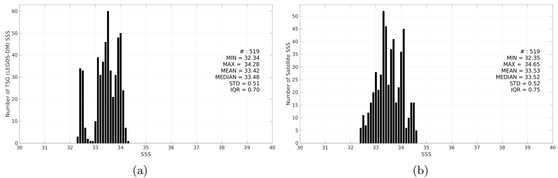
Figure 3: Histograms of SSS from TSG (LEGOS-DM) (a) and SMAP SSS L2 v6 (RSS) (b) considering all match-up pairs per bins of 0.1 over the Bay of Bengal Pi-MEP region and for the full satellite product period.
