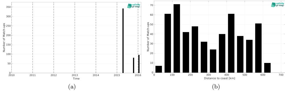
Figure 2: Number of match-ups between TSG (LEGOS-DM) and SMAP SSS L2 v6 (RSS) SSS as a function of time (a) and as function of the distance to coast (b) over the Bay of Bengal Pi-MEP region and for the full satellite product period.
