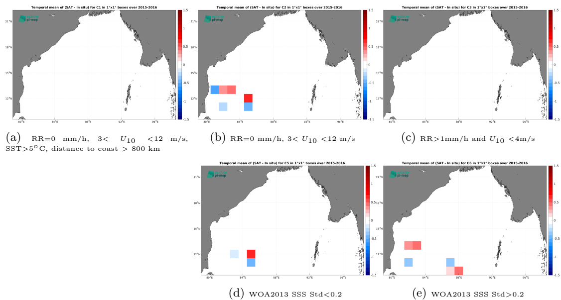
Figure 14: Temporal mean gridded over spatial boxes of size 1^\circ \times 1^\circ of \Delta SSS (SMAP SSS L2 v6 - 40 km (RSS) - TSG (LEGOS-DM)) for 5 different subdatasets corresponding to:RR=0 mm/h, 3 < U_{10} < 12 m/s, SST >5^\circ\text{C} , distance to coast > 800 km (a), RR=0 mm/h, 3 < U_{10} < 12 m/s (b), RR >1 mm/h and U_{10} < 4 m/s (c), WOA2013 SSS Std <0.2 (d), WOA2013 SSS Std >0.2 (e).
