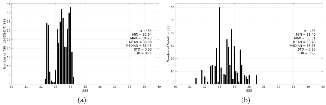
Figure 3: Histograms of SSS from TSG (LEGOS-DM) (a) and SMAP SSS L2 v6 - 40 km (RSS) (b) considering all match-up pairs per bins of 0.1 over the Bay of Bengal Pi-MEP region and for the full satellite product period.
