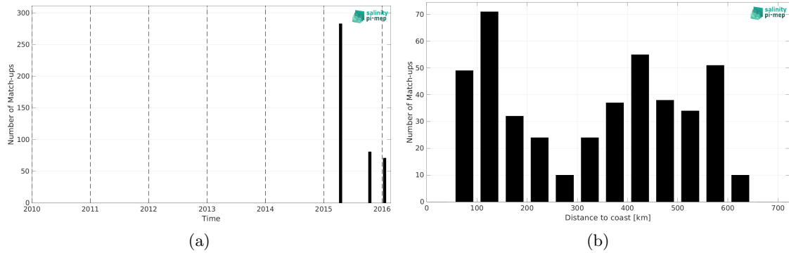
Figure 2: Number of match-ups between TSG (LEGOS-DM) and SMAP SSS L2 v6 - 40 km (RSS) SSS as a function of time (a) and as function of the distance to coast (b) over the Bay of Bengal Pi-MEP region and for the full satellite product period.
