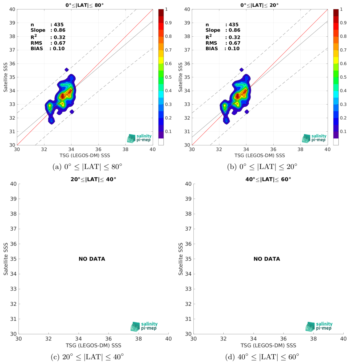
Figure 10: Contour maps of the concentration of SMAP SSS L2 v6 - 40 km (RSS) SSS (y-axis) versus TSG (LEGOS-DM) SSS (x-axis) at match-up pairs for different latitude bands. For each plot, the red line shows x=y . The black thin and dashed lines indicate a linear fit through the data cloud and the \pm 95\% confidence levels, respectively. The number match-up pairs n , the slope and R^2 coefficient of the linear fit, the root mean square (RMS) and the mean bias between satellite and in situ data are indicated for each latitude band in each plots.
