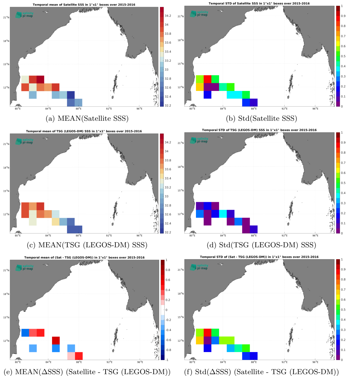
Figure 7: Temporal mean (left) and Std (right) of SSS from SMAP SSS L2 v6 - 40 km (RSS) (top), TSG (LEGOS-DM) (middle), and of \Delta SSS (Satellite - TSG (LEGOS-DM)). Only match-up pairs are used to generate these maps.
