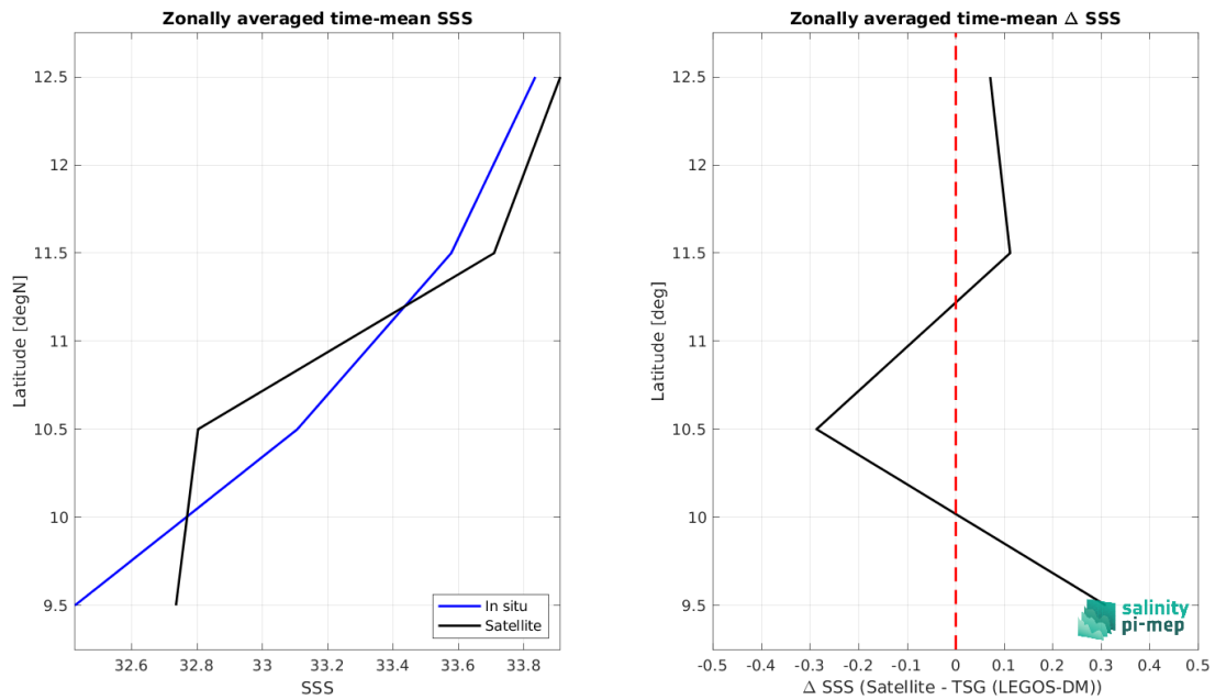
Figure 9: Left panel: Zonal mean SSS from SMAP SSS L2 v6 - 40 km (RSS) satellite product (black) and from TSG (LEGOS-DM) (blue). Right panel: Zonal mean of \Delta SSS (Satellite - TSG (LEGOS-DM)) for all the collected Pi-MEP match-up pairs estimated over the full satellite product period.
