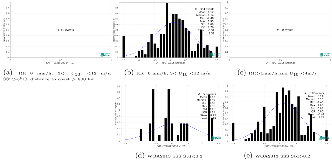
Figure 15: Normalized histogram of \Delta SSS (SMAP SSS L2 v6 - 40 km (RSS) - TSG (LEGOS-DM)) for 5 different subdatasets corresponding to: RR=0 mm/h, 3 < U_{10} < 12 m/s, SST > 5°C, distance to coast > 800 km (a), RR=0 mm/h, 3 < U_{10} < 12 m/s (b), RR > 1mm/h and U_{10} < 4 m/s (c), WOA2013 SSS Std < 0.2 (d), WOA2013 SSS Std > 0.2 (e).
