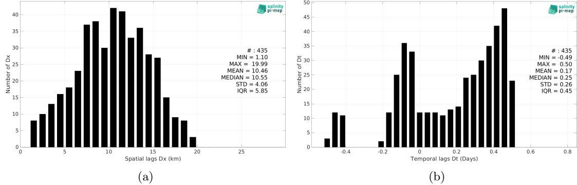
Figure 6: Histograms of the spatial (a) and temporal (b) lags between the location/time of the TSG (LEGOS-DM) measurement and the date of the corresponding SMAP SSS L2 v6 - 40 km (RSS) SSS pixel.
