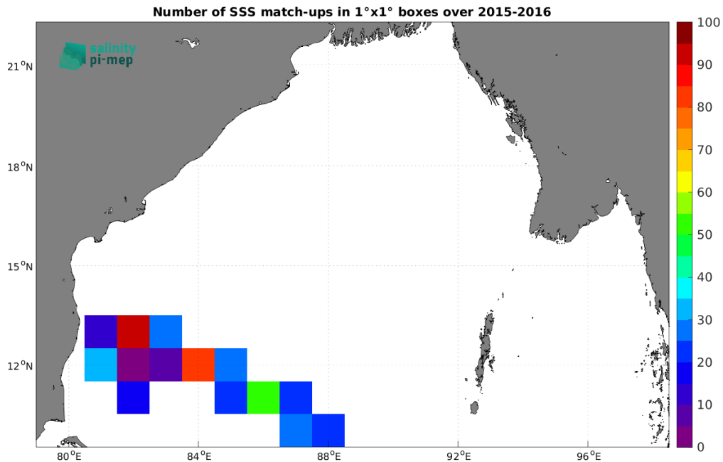
Figure 5: Number of SSS match-ups between TSG (LEGOS-DM) SSS and the SMAP SSS L2 v6 - 40 km (RSS) SSS product for the Bay of Bengal Pi-MEP region over 1^\circ \times 1^\circ boxes and for the full satellite product period.
