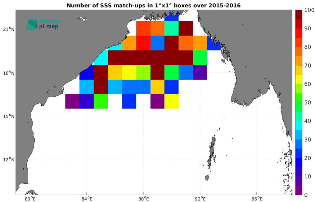
Figure 4: Number of SSS match-ups between Surface drifters SSS and the SMAP SSS L2 v6 - 40 km (RSS) SSS product for the Bay of Bengal Pi-MEP region over 1^\circ \times 1^\circ boxes and for the full satellite product period.
