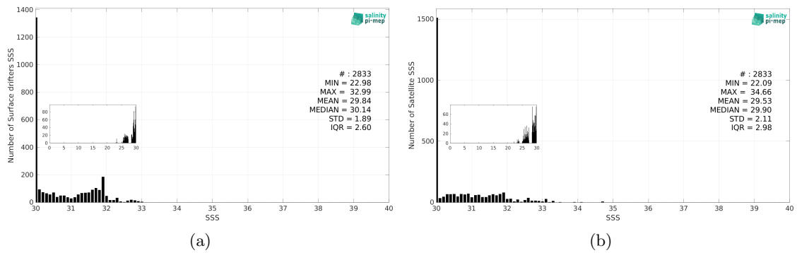
Figure 3: Histograms of SSS from Surface drifters (a) and SMAP SSS L2 v6 - 40 km (RSS) (b) considering all match-up pairs per bins of 0.1 over the Bay of Bengal Pi-MEP region and for the full satellite product period.
