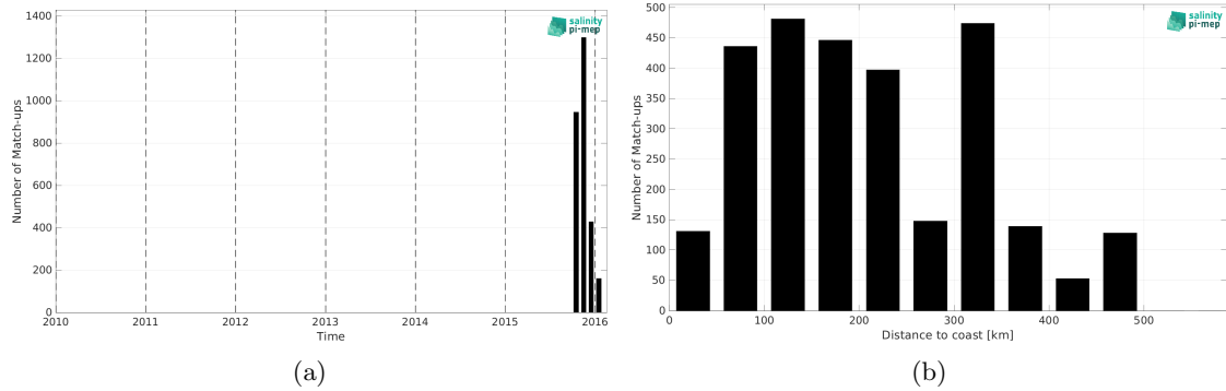
Figure 2: Number of match-ups between Surface drifters and SMAP SSS L2 v6 - 40 km (RSS) SSS as a function of time (a) and as function of the distance to coast (b) over the Bay of Bengal Pi-MEP region and for the full satellite product period.
