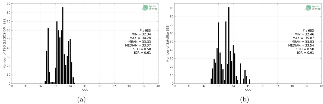
Figure 2: Histograms of SSS from TSG (LEGOS-DM) (a) and SMAP SSS L2 v5 (RSS) (b) considering all match-up pairs per bins of 0.1 over the Bay of Bengal Pi-MEP region and for the full satellite product period.
