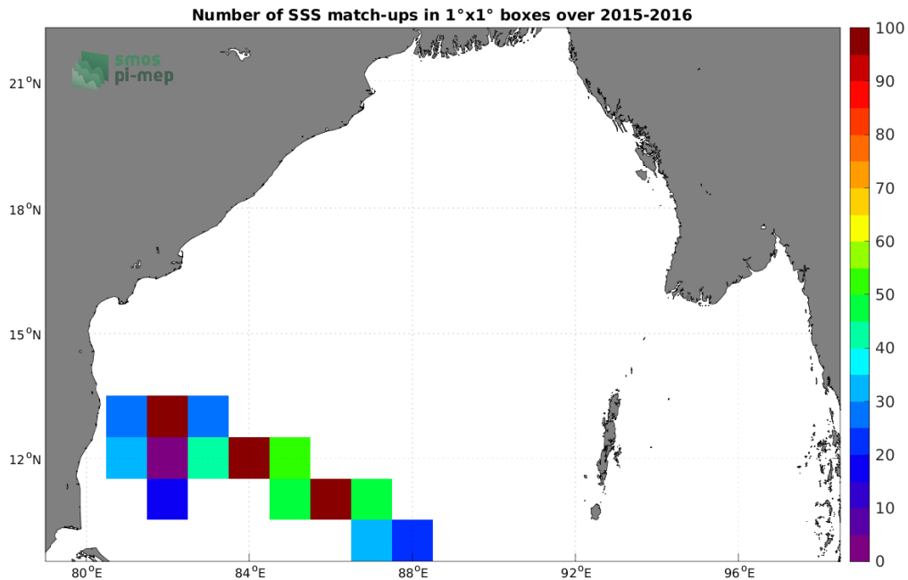
Figure 4: Number of SSS match-ups between TSG (LEGOS-DM) SSS and the SMAP SSS L2 v5 (RSS) SSS product for the Bay of Bengal Pi-MEP region over 1^\circ \times 1^\circ boxes and for the full satellite product period.
