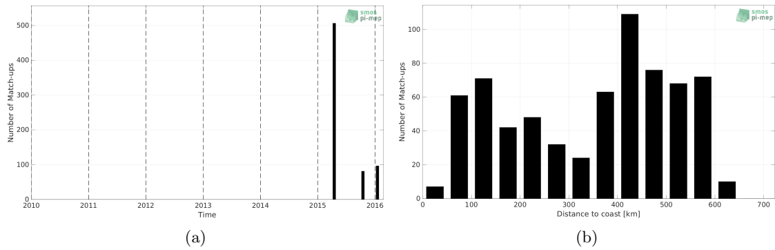
Figure 1: Number of match-ups between TSG (LEGOS-DM) and SMAP SSS L2 v5 (RSS) SSS as a function of time (a) and as function of the distance to coast (b) over the Bay of Bengal Pi-MEP region and for the full satellite product period.
