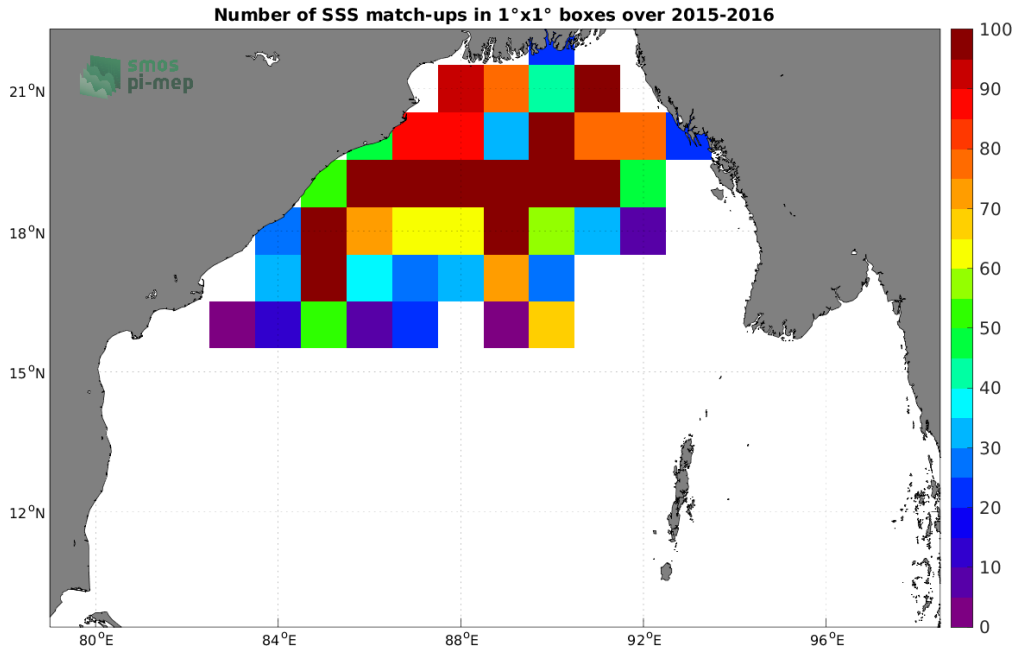
Figure 3: Number of SSS match-ups between Surface drifters SSS and the SMAP SSS L2 v5 (RSS) SSS product for the Bay of Bengal Pi-MEP region over 1^\circ \times 1^\circ boxes and for the full satellite product period.
