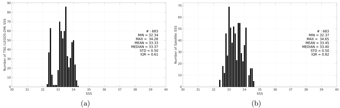
Figure 3: Histograms of SSS from TSG (LEGOS-DM) (a) and SMAP SSS L2 v5.3 (RSS) (b) considering all match-up pairs per bins of 0.1 over the Bay of Bengal Pi-MEP region and for the full satellite product period.
