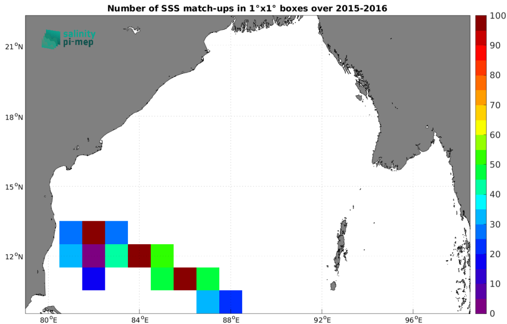
Figure 5: Number of SSS match-ups between TSG (LEGOS-DM) SSS and the SMAP SSS L2 v5.3 (RSS) SSS product for the Bay of Bengal Pi-MEP region over 1^\circ \times 1^\circ boxes and for the full satellite product period.
