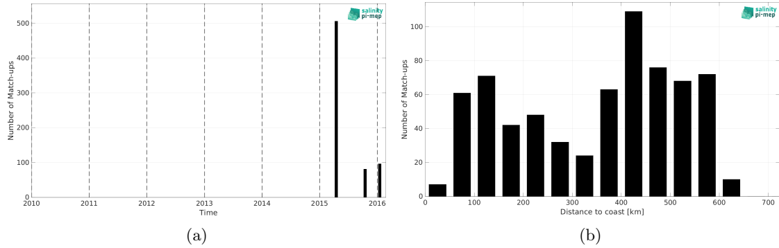
Figure 2: Number of match-ups between TSG (LEGOS-DM) and SMAP SSS L2 v5.3 (RSS) SSS as a function of time (a) and as function of the distance to coast (b) over the Bay of Bengal Pi-MEP region and for the full satellite product period.
