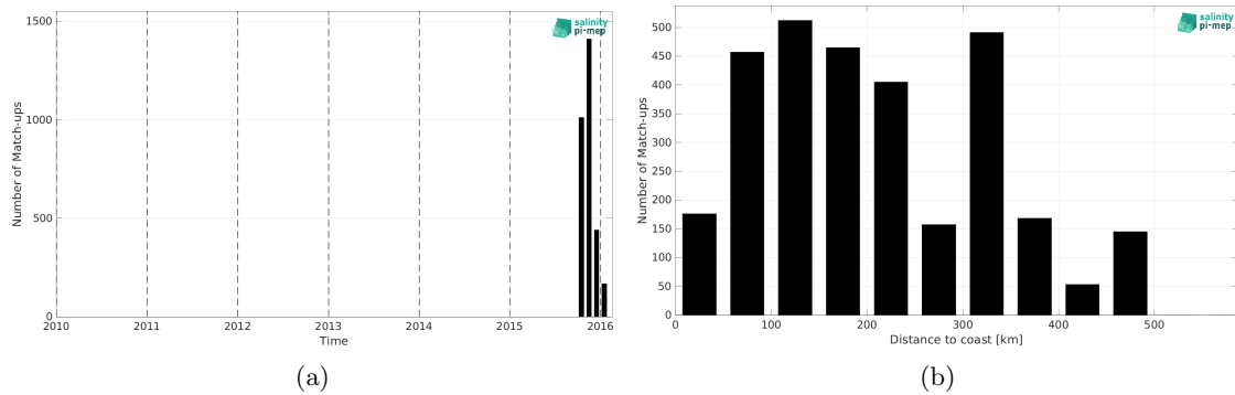
Figure 2: Number of match-ups between Surface drifters and SMAP SSS L2 v5.3 (RSS) SSS as a function of time (a) and as function of the distance to coast (b) over the Bay of Bengal Pi-MEP region and for the full satellite product period.
