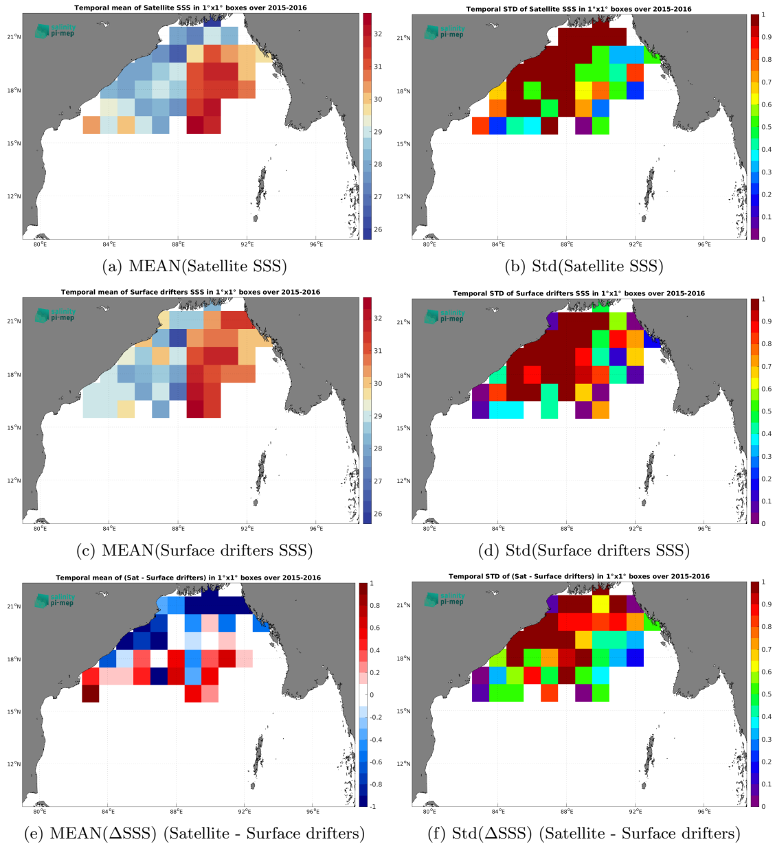
Figure 6: Temporal mean (left) and Std (right) of SSS from SMAP SSS L2 v5.3 (RSS) (top), Surface drifters (middle), and of \Delta SSS (Satellite - Surface drifters). Only match-up pairs are used to generate these maps.
