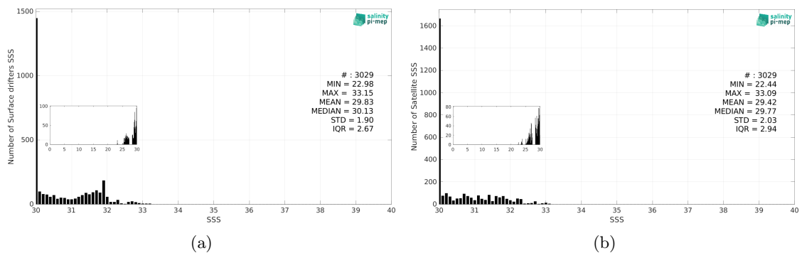
Figure 3: Histograms of SSS from Surface drifters (a) and SMAP SSS L2 v5.3 (RSS) (b) considering all match-up pairs per bins of 0.1 over the Bay of Bengal Pi-MEP region and for the full satellite product period.
