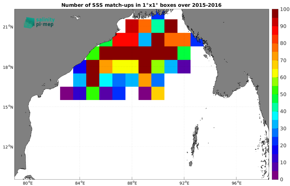
Figure 4: Number of SSS match-ups between Surface drifters SSS and the SMAP SSS L2 v5.3 (RSS) SSS product for the Bay of Bengal Pi-MEP region over 1^\circ \times 1^\circ boxes and for the full satellite product period.
