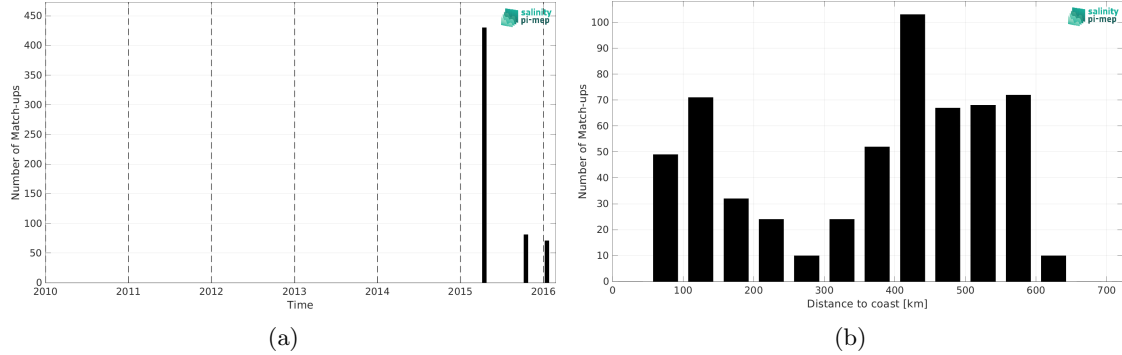
Figure 2: Number of match-ups between TSG (LEGOS-DM) and SMAP SSS L2 v5.3 - 40 km (RSS) SSS as a function of time (a) and as function of the distance to coast (b) over the Bay of Bengal Pi-MEP region and for the full satellite product period.
