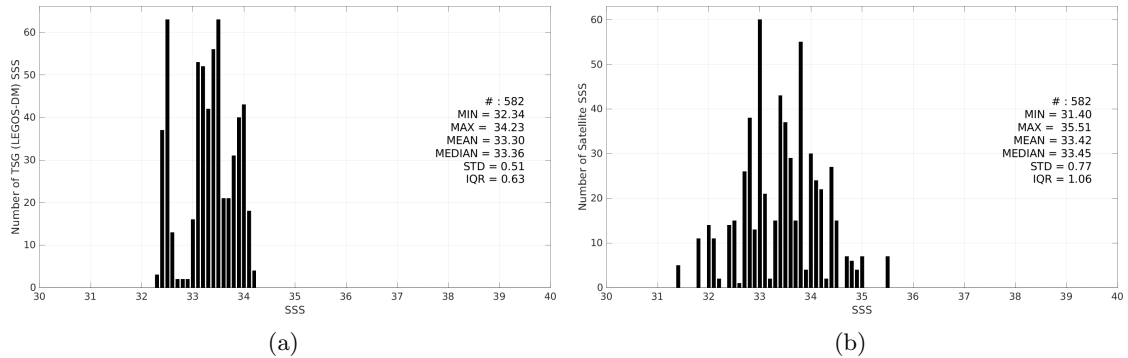
Figure 3: Histograms of SSS from TSG (LEGOS-DM) (a) and SMAP SSS L2 v5.3 - 40 km (RSS) (b) considering all match-up pairs per bins of 0.1 over the Bay of Bengal Pi-MEP region and for the full satellite product period.
