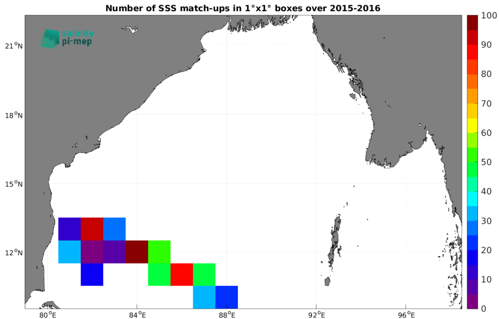
Figure 5: Number of SSS match-ups between TSG (LEGOS-DM) SSS and the SMAP SSS L2 v5.3 - 40 km (RSS) SSS product for the Bay of Bengal Pi-MEP region over 1^\circ \times 1^\circ boxes and for the full satellite product period.
