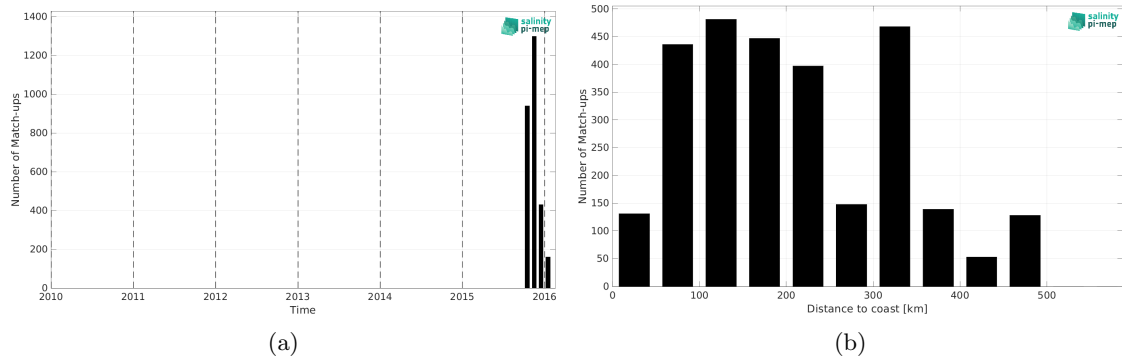
Figure 2: Number of match-ups between Surface drifters and SMAP SSS L2 v5.3 - 40 km (RSS) SSS as a function of time (a) and as function of the distance to coast (b) over the Bay of Bengal Pi-MEP region and for the full satellite product period.
