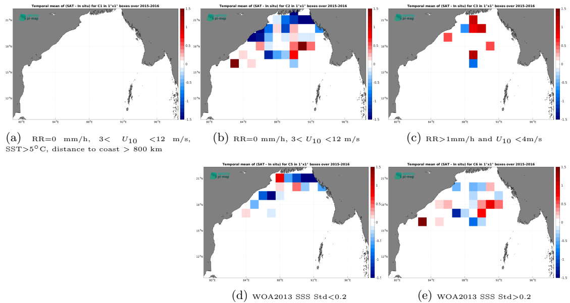
Figure 13: Temporal mean gridded over spatial boxes of size 1^\circ \times 1^\circ of \Delta SSS (SMAP SSS L2 v5.3 - 40 km (RSS) - Surface drifters) for 5 different subdatasets corresponding to:RR=0 mm/h, 3 < U_{10} < 12 m/s, SST >5^\circ\text{C} , distance to coast > 800 km (a), RR=0 mm/h, 3 < U_{10} < 12 m/s (b), RR >1 mm/h and U_{10} < 4 m/s (c), WOA2013 SSS Std <0.2 (d), WOA2013 SSS Std >0.2 (e).
