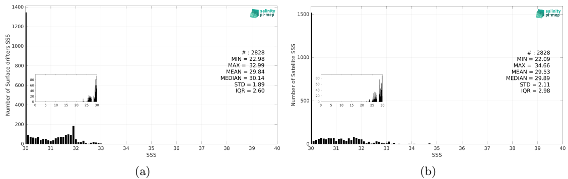
Figure 3: Histograms of SSS from Surface drifters (a) and SMAP SSS L2 v5.3 - 40 km (RSS) (b) considering all match-up pairs per bins of 0.1 over the Bay of Bengal Pi-MEP region and for the full satellite product period.
