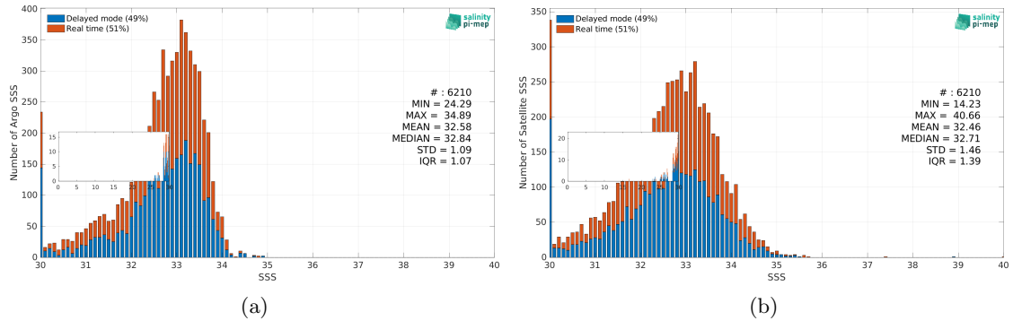
Figure 3: Histograms of SSS from Argo (a) and SMAP SSS L2 v5.3 - 40 km (RSS) (b) considering all match-up pairs per bins of 0.1 over the Bay of Bengal Pi-MEP region and for the full satellite product period.
