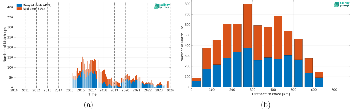
Figure 2: Number of match-ups between Argo and SMAP SSS L2 v5.3 - 40 km (RSS) SSS as a function of time (a) and as function of the distance to coast (b) over the Bay of Bengal Pi-MEP region and for the full satellite product period.
