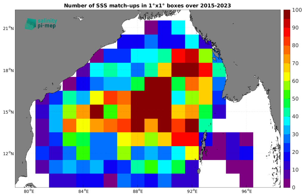
Figure 5: Number of SSS match-ups between Argo SSS and the SMAP SSS L2 v5.3 - 40 km (RSS) SSS product for the Bay of Bengal Pi-MEP region over 1°×1° boxes and for the full satellite product period.
