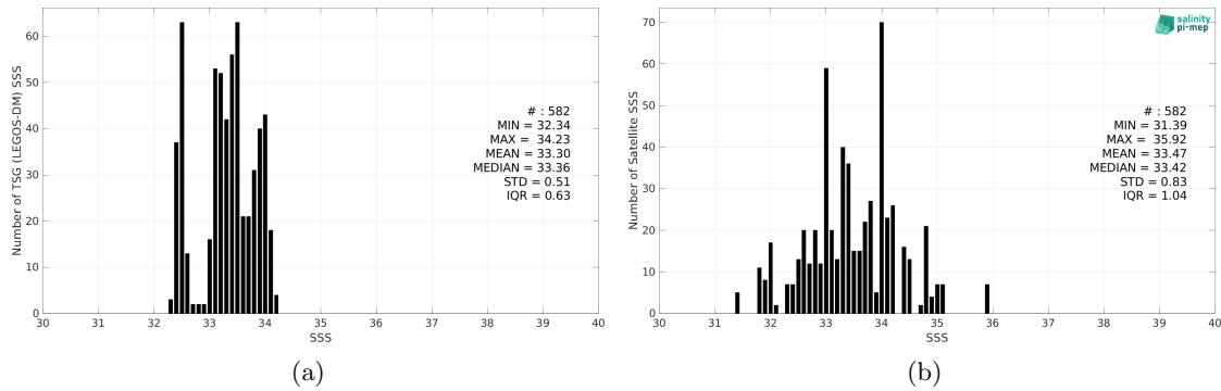
Figure 2: Histograms of SSS from TSG (LEGOS-DM) (a) and SMAP SSS L2 v5 - 40 km (RSS) (b) considering all match-up pairs per bins of 0.1 over the Bay of Bengal Pi-MEP region and for the full satellite product period.
