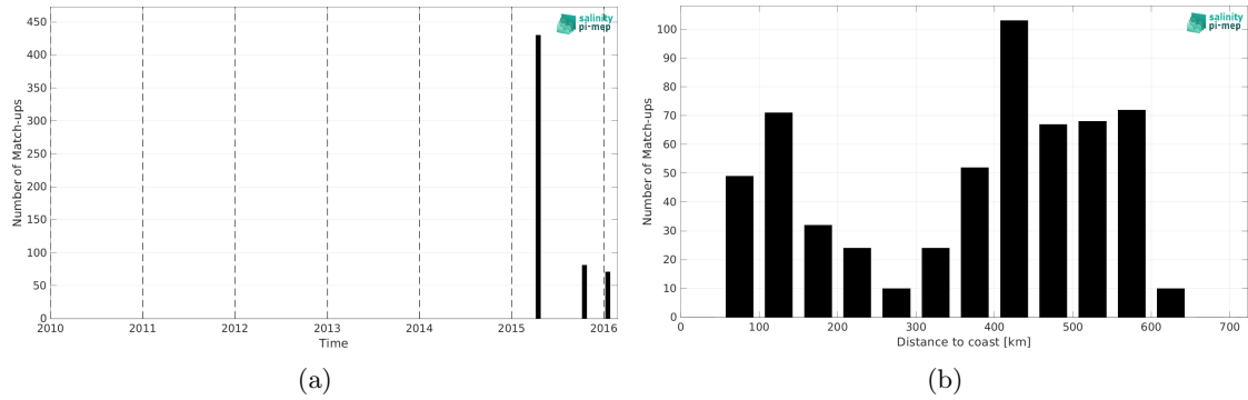
Figure 1: Number of match-ups between TSG (LEGOS-DM) and SMAP SSS L2 v5 - 40 km (RSS) SSS as a function of time (a) and as function of the distance to coast (b) over the Bay of Bengal Pi-MEP region and for the full satellite product period.
