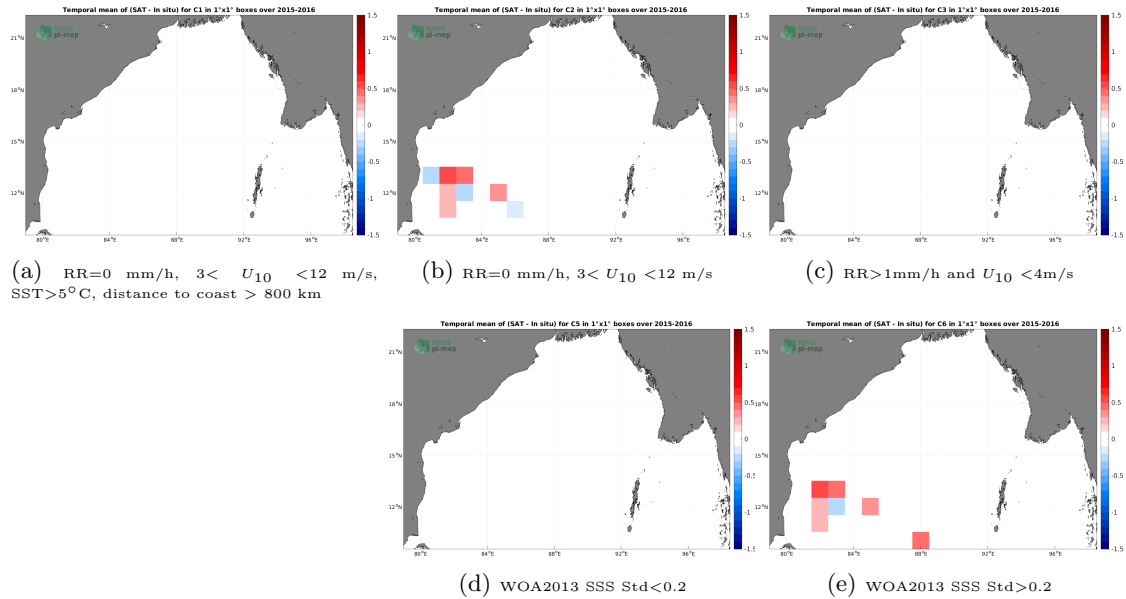
Figure 12: Temporal mean gridded over spatial boxes of size 1^\circ \times 1^\circ of \Delta\text{SSS} (SMAP SSS L2 v5 - 40 km (RSS) - TSG (LEGOS-DM)) for 5 different subdatasets corresponding to:RR=0 mm/h, 3 < U_{10} < 12 m/s, SST >5^\circ\text{C} , distance to coast > 800 km (a), RR=0 mm/h, 3 < U_{10} < 12 m/s (b), RR >1 mm/h and U_{10} < 4 m/s (c), WOA2013 SSS Std <0.2 (d), WOA2013 SSS Std >0.2 (e).
