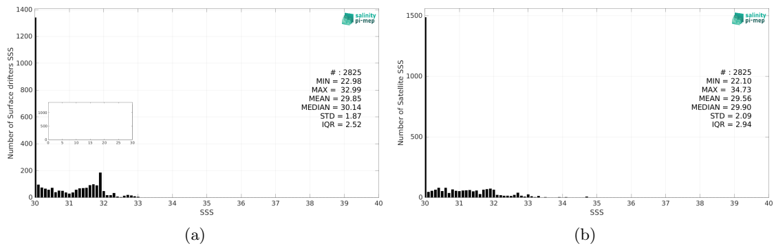
Figure 2: Histograms of SSS from Surface drifters (a) and SMAP SSS L2 v5 - 40 km (RSS) (b) considering all match-up pairs per bins of 0.1 over the Bay of Bengal Pi-MEP region and for the full satellite product period.
