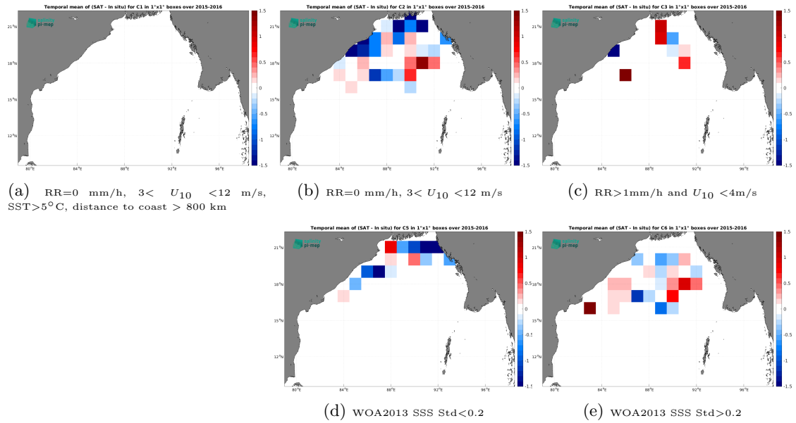
Figure 11: Temporal mean gridded over spatial boxes of size 1^\circ \times 1^\circ of \Delta SSS (SMAP SSS L2 v5 - 40 km (RSS) - Surface drifters) for 5 different subdatasets corresponding to:RR=0 mm/h, 3 < U_{10} < 12 m/s, SST > 5^\circ\text{C} , distance to coast > 800 km (a), RR=0 mm/h, 3 < U_{10} < 12 m/s (b), RR > 1 mm/h and U_{10} < 4 m/s (c), WOA2013 SSS Std < 0.2 (d), WOA2013 SSS Std > 0.2 (e).
