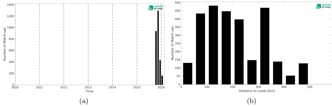
Figure 1: Number of match-ups between Surface drifters and SMAP SSS L2 v5 - 40 km (RSS) SSS as a function of time (a) and as function of the distance to coast (b) over the Bay of Bengal Pi-MEP region and for the full satellite product period.
