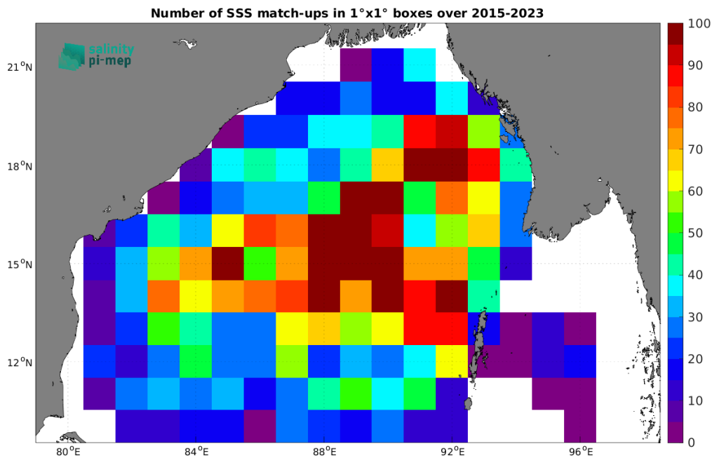
Figure 4: Number of SSS match-ups between Argo SSS and the SMAP SSS L2 v5 - 40 km (RSS) SSS product for the Bay of Bengal Pi-MEP region over 1^\circ \times 1^\circ boxes and for the full satellite product period.
