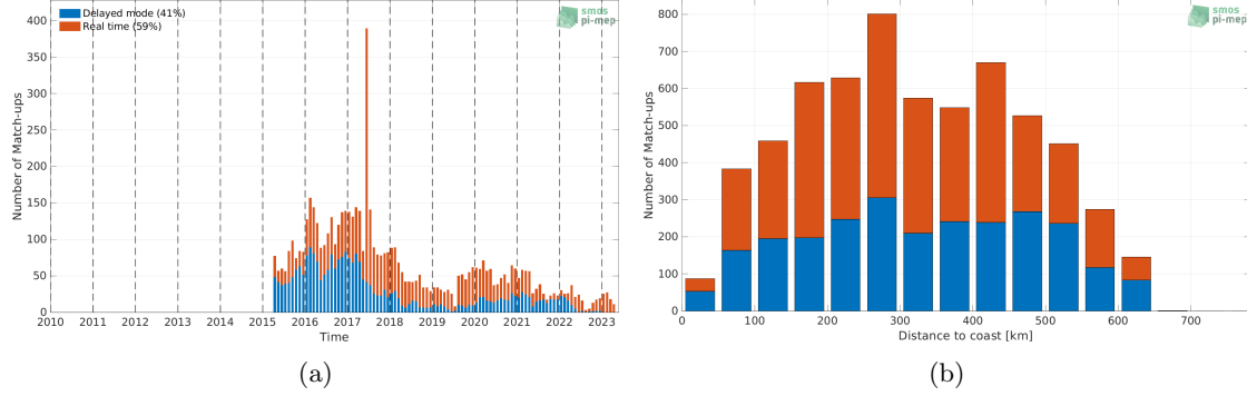
Figure 1: Number of match-ups between Argo and SMAP SSS L2 v5 - 40 km (RSS) SSS as a function of time (a) and as function of the distance to coast (b) over the Bay of Bengal Pi-MEP region and for the full satellite product period.
