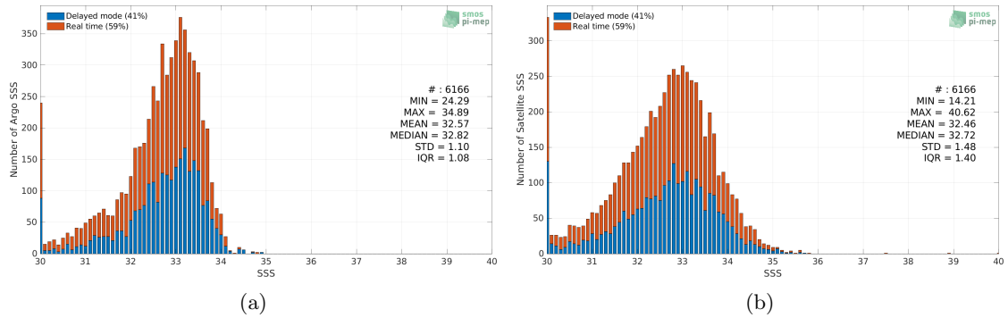
Figure 2: Histograms of SSS from Argo (a) and SMAP SSS L2 v5 - 40 km (RSS) (b) considering all match-up pairs per bins of 0.1 over the Bay of Bengal Pi-MEP region and for the full satellite product period.
