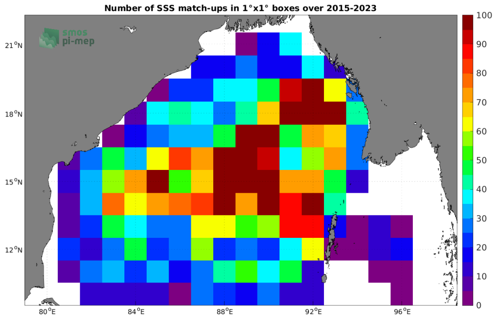
Figure 4: Number of SSS match-ups between Argo SSS and the SMAP SSS L2 v5 - 40 km (RSS) SSS product for the Bay of Bengal Pi-MEP region over 1°x1° boxes and for the full satellite product period.
