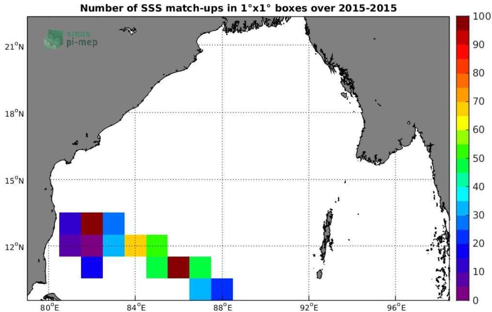
Figure 4: Number of SSS match-ups between TSG-LEGOS-DM SSS and the SMAP-L2-RSS-V4 SSS product for the Bay of Bengal Pi-MEP region over 1°x1° boxes and for the full satellite product period.
