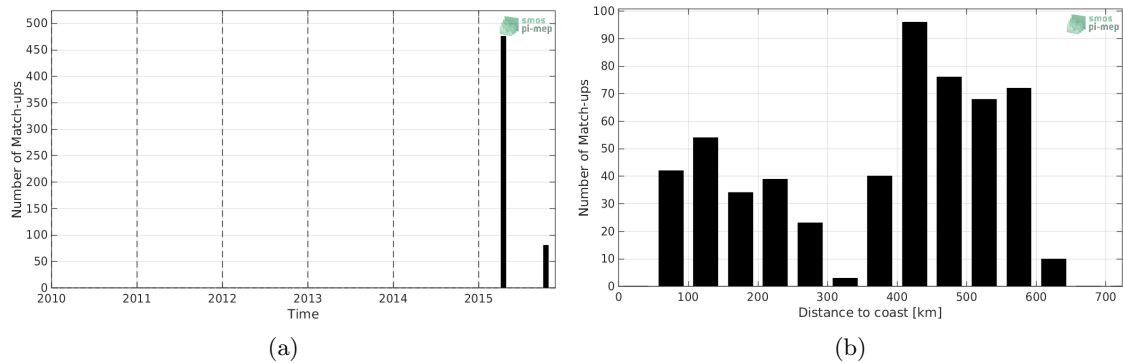
Figure 1: Number of match-ups between TSG-LEGOS-DM and SMAP-L2-RSS-V4 SSS as a function of time (a) and as function of the distance to coast (b) over the Bay of Bengal Pi-MEP region and for the full satellite product period.
