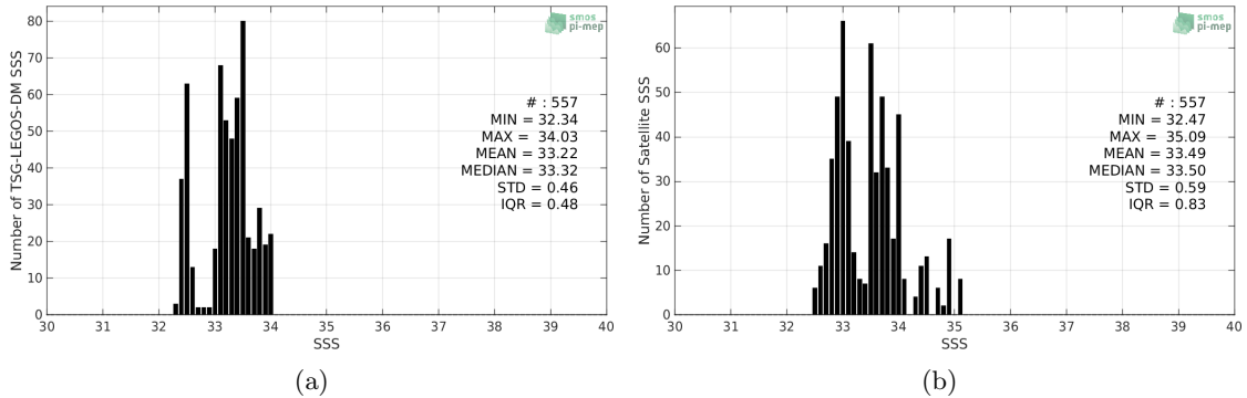
Figure 2: Histograms of SSS from TSG-LEGOS-DM (a) and SMAP-L2-RSS-V4 (b) considering all match-up pairs per bins of 0.1 over the Bay of Bengal Pi-MEP region and for the full satellite product period.
