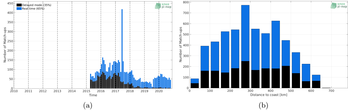
Figure 1: Number of match-ups between Argo and SMAP SSS L2 v4 (RSS) SSS as a function of time (a) and as function of the distance to coast (b) over the Bay of Bengal Pi-MEP region and for the full satellite product period.
