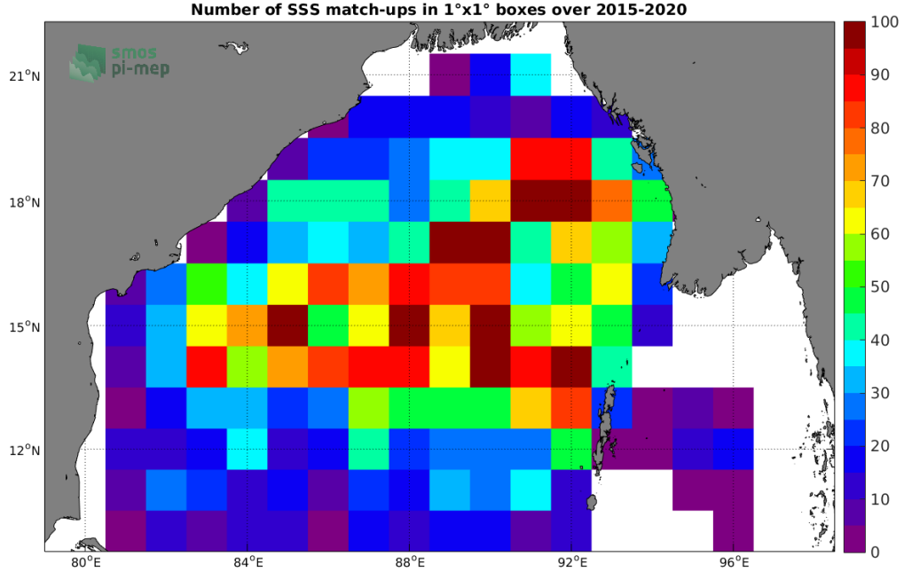
Figure 4: Number of SSS match-ups between Argo SSS and the SMAP SSS L2 v4 (RSS) SSS product for the Bay of Bengal Pi-MEP region over 1^\circ \times 1^\circ boxes and for the full satellite product period.
