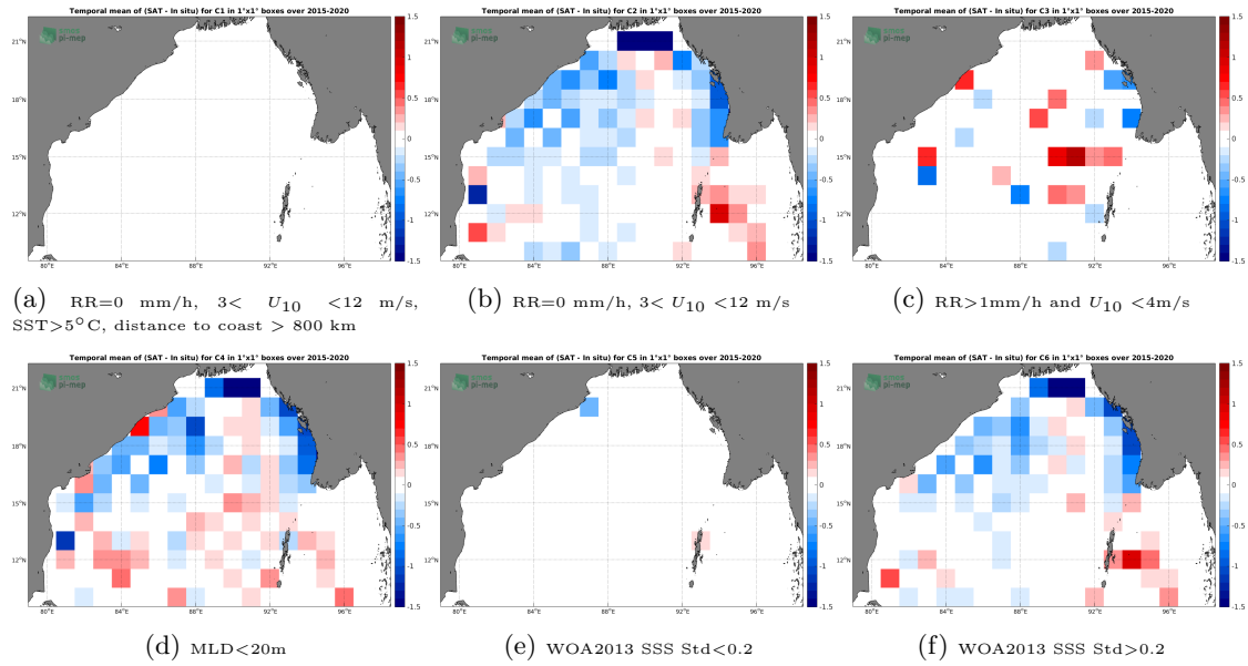
Figure 12: Temporal mean gridded over spatial boxes of size 1^\circ \times 1^\circ of \Delta SSS (SMAP SSS L2 v4 (RSS) - Argo) for 6 different subdatasets corresponding to: RR=0 mm/h, 3 < U_{10} < 12 m/s, SST > 5^\circ C , distance to coast > 800 km (a), RR=0 mm/h, 3 < U_{10} < 12 m/s (b), RR > 1 mm/h and U_{10} < 4 m/s (c), MLD < 20 m (d), WOA2013 SSS Std < 0.2 (e), WOA2013 SSS Std > 0.2 (f).
