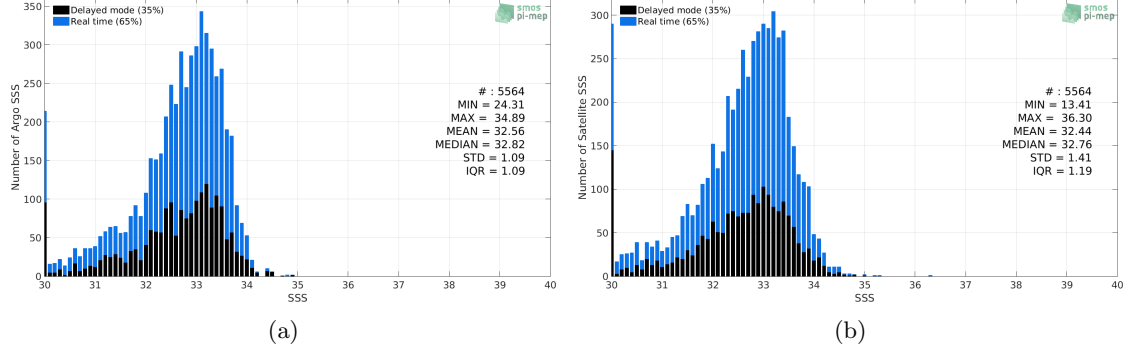
Figure 2: Histograms of SSS from Argo (a) and SMAP SSS L2 v4 (RSS) (b) considering all match-up pairs per bins of 0.1 over the Bay of Bengal Pi-MEP region and for the full satellite product period.
