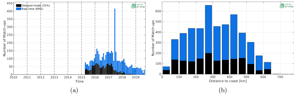
Figure 1: Number of match-ups between Argo and SMAP-L2-RSS-V4 SSS as a function of time (a) and as function of the distance to coast (b) over the Bay of Bengal Pi-MEP region and for the full satellite product period.
