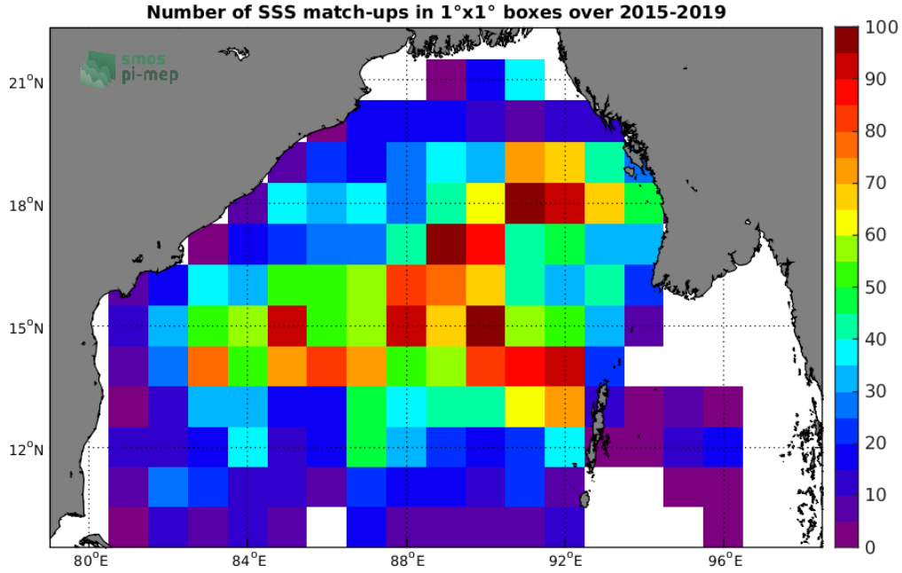
Figure 4: Number of SSS match-ups between Argo SSS and the SMAP-L2-RSS-V4 SSS product for the Bay of Bengal Pi-MEP region over 1^\circ \times 1^\circ boxes and for the full satellite product period.
