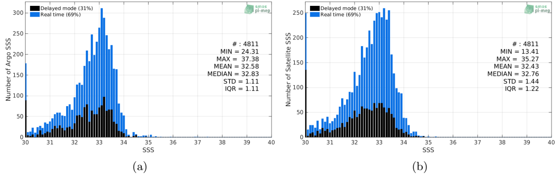
Figure 2: Histograms of SSS from Argo (a) and SMAP-L2-RSS-V4 (b) considering all match-up pairs per bins of 0.1 over the Bay of Bengal Pi-MEP region and for the full satellite product period.
