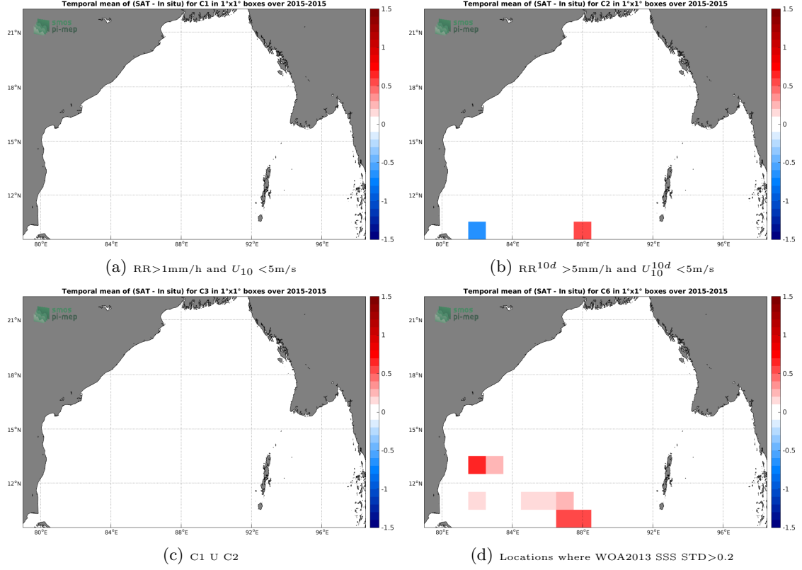
Figure 12: Temporal mean gridded over spatial boxes of size 1^\circ \times 1^\circ of \Delta SSS (SMAP-L2-RSS-V3-70KM - TSG-LEGOS-DM) for 4 different subdatasets corresponding to: RR > 1\text{mm/h} and U_{10} < 5\text{m/s} (a), RR^{10d} > 5\text{mm/h} and U_{10}^{10d} < 5\text{m/s} (b), C1 U C2 (c), Locations where WOA2013 SSS STD > 0.2 (d).
