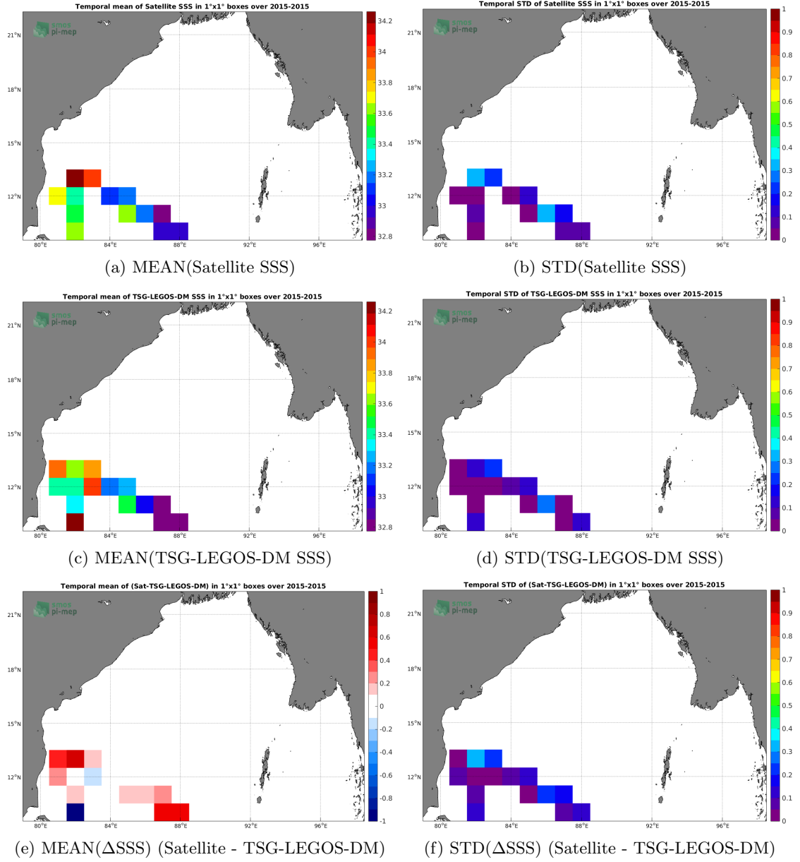
Figure 6: Temporal mean (left) and STD (right) of SSS from SMAP-L2-RSS-V3-70KM (top), TSG-LEGOS-DM (middle), and of \Delta SSS (Satellite - TSG-LEGOS-DM). Only match-up pairs are used to generate these maps.
