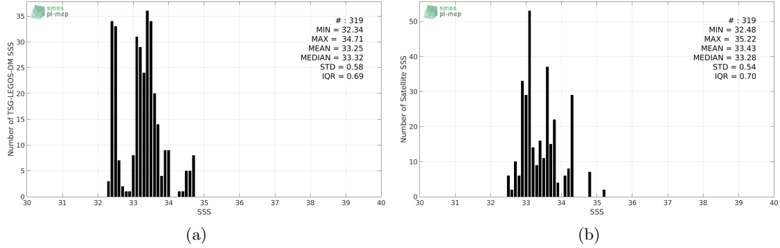
Figure 2: Histograms of SSS from TSG-LEGOS-DM (a) and SMAP-L2-RSS-V3-70KM (b) considering all match-up pairs per bins of 0.1 over the Bay of Bengal Pi-MEP region and for the full satellite product period.
