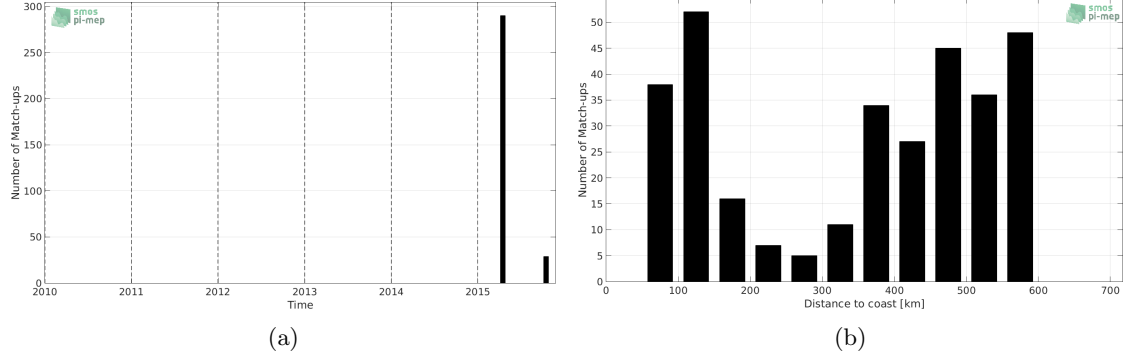
Figure 1: Number of match-ups between TSG-LEGOS-DM and SMAP-L2-RSS-V3-70KM SSS as a function of time (a) and as function of the distance to coast (b) over the Bay of Bengal Pi-MEP region and for the full satellite product period.
