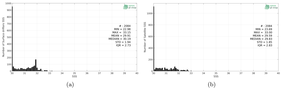
Figure 2: Histograms of SSS from Surface drifters (a) and SMAP-L2-RSS-V3-70KM (b) considering all match-up pairs per bins of 0.1 over the Bay of Bengal Pi-MEP region and for the full satellite product period.
