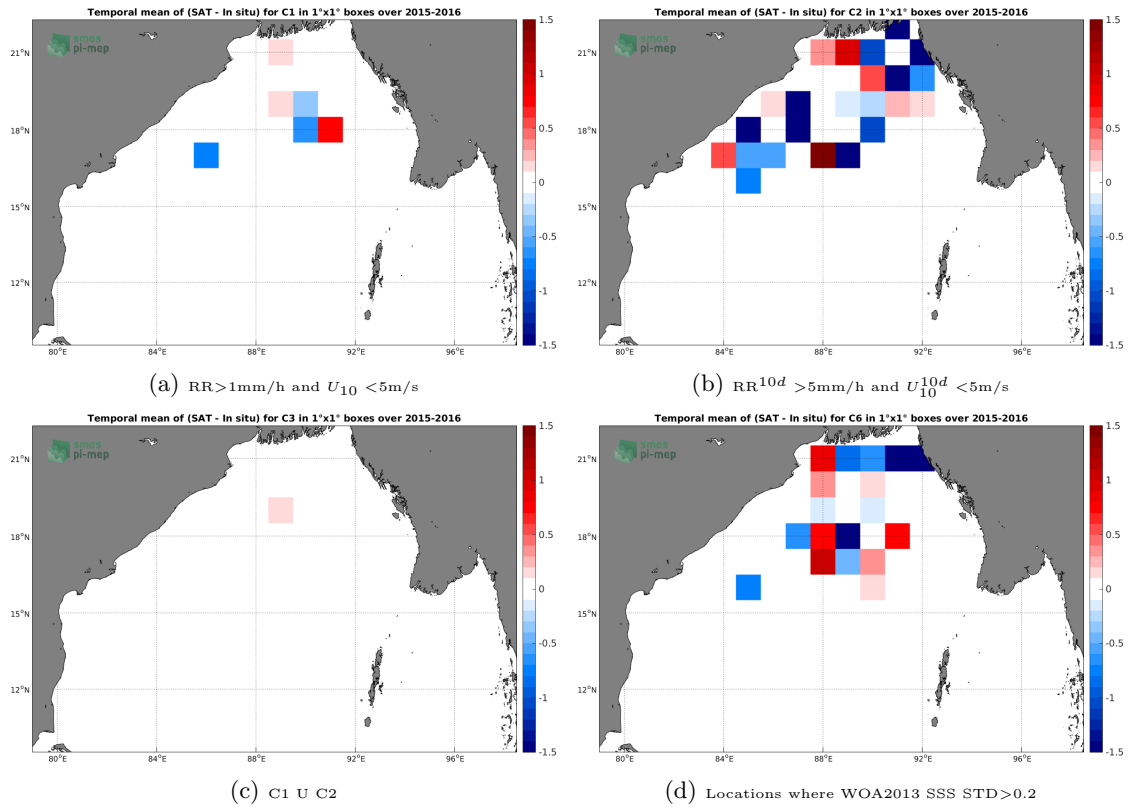
Figure 11: Temporal mean gridded over spatial boxes of size 1^\circ \times 1^\circ of \Delta SSS (SMAP-L2-RSS-V3-70KM - Surface drifters) for 4 different subdatasets corresponding to:RR > 1 mm/h and U_{10} < 5 m/s (a), RR^{10d} > 5 mm/h and U_{10}^{10d} < 5 m/s (b), C1 U C2 (c),Locations where WOA2013 SSS STD > 0.2 (d).
