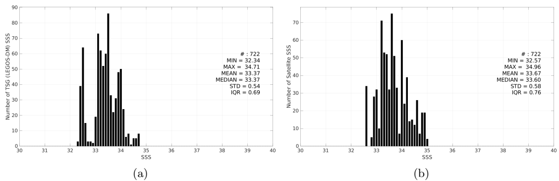
Figure 3: Histograms of SSS from TSG (LEGOS-DM) (a) and SMAP SSS L2 v5.0 (JPL) (b) considering all match-up pairs per bins of 0.1 over the Bay of Bengal Pi-MEP region and for the full satellite product period.
