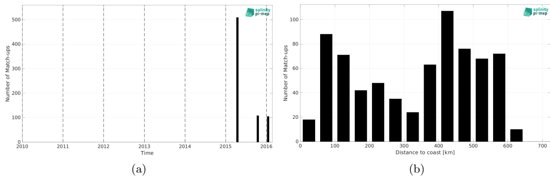
Figure 2: Number of match-ups between TSG (LEGOS-DM) and SMAP SSS L2 v5.0 (JPL) SSS as a function of time (a) and as function of the distance to coast (b) over the Bay of Bengal Pi-MEP region and for the full satellite product period.
