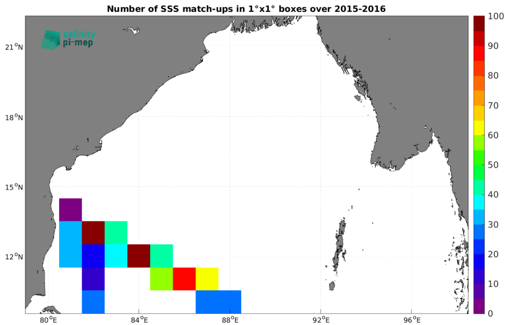
Figure 5: Number of SSS match-ups between TSG (LEGOS-DM) SSS and the SMAP SSS L2 v5.0 (JPL) SSS product for the Bay of Bengal Pi-MEP region over 1^\circ \times 1^\circ boxes and for the full satellite product period.
