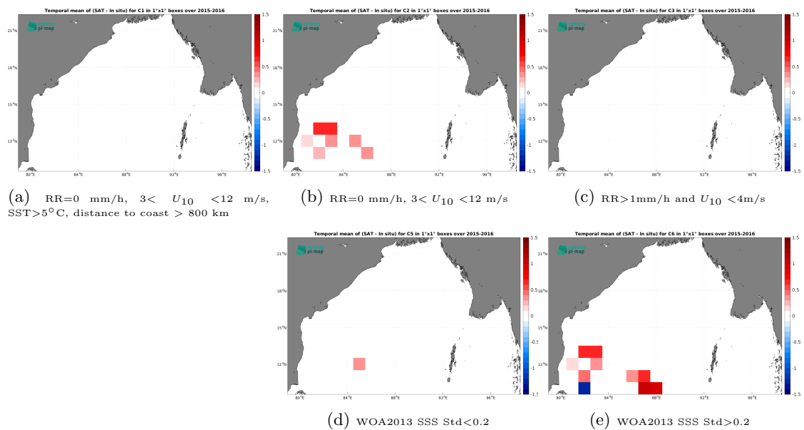
Figure 14: Temporal mean gridded over spatial boxes of size 1^\circ \times 1^\circ of \Delta SSS (SMAP SSS L2 v5.0 (JPL) - TSG (LEGOS-DM)) for 5 different subdatasets corresponding to:RR=0 mm/h, 3 < U_{10} < 12 m/s, SST>5°C, distance to coast > 800 km (a), RR=0 mm/h, 3 < U_{10} < 12 m/s (b), RR>1mm/h and U_{10} < 4 m/s (c), WOA2013 SSS Std<0.2 (d), WOA2013 SSS Std>0.2 (e).
